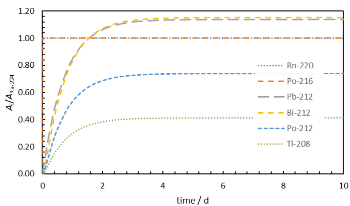
Figure 2. Solving the Bateman equations illustrates that the relatively long-lived ^{224}\text{Ra} progeny, ^{212}\text{Pb} ( T_{1/2} = 10.6 h), leads to a long equilibration period. In the top panel, activities are given relative to the initial ^{224}\text{Ra} activity, showing that, by the time equilibrium is reached, the ^{224}\text{Ra} activity is less than 22 % of its initial value. In the bottom panel, activities for the progeny are shown relative to the ^{224}\text{Ra} activity at the same time, as in Figure 1.
