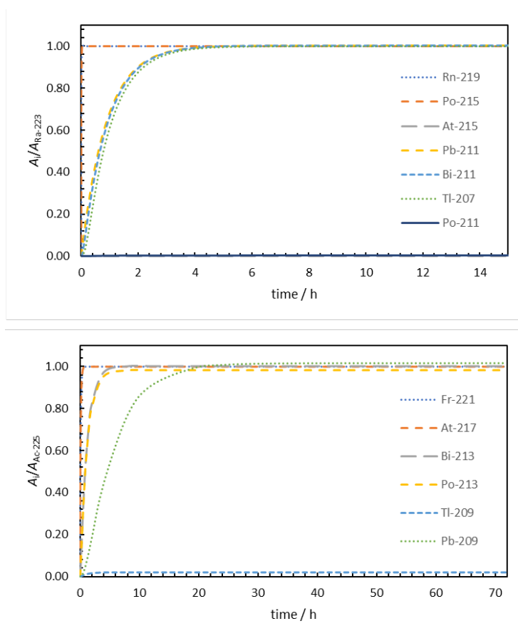
Figure 1. Solving the Bateman equations illustrates that equilibrium is achieved more rapidly for ^{223}\text{Ra} (longest-lived progeny is ^{211}\text{Pb} , T_{1/2} = 36.1 min) than for ^{225}\text{Ac} (longest-lived progeny is ^{209}\text{Pb} , T_{1/2} = 3.28 h). Activities for the progeny are shown relative to the parent activity at the same time.
