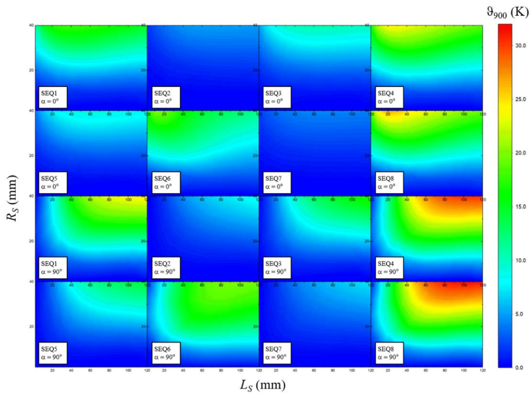
Figure E2. Maximum \vartheta_{900} in CoCrMo-alloy prolate spheroid models in ASTM gel as a function of radius R_S , semi-height R_S , incident angle \alpha of the GC field with respect to R_L and GC sequence number (as described in table 1).
