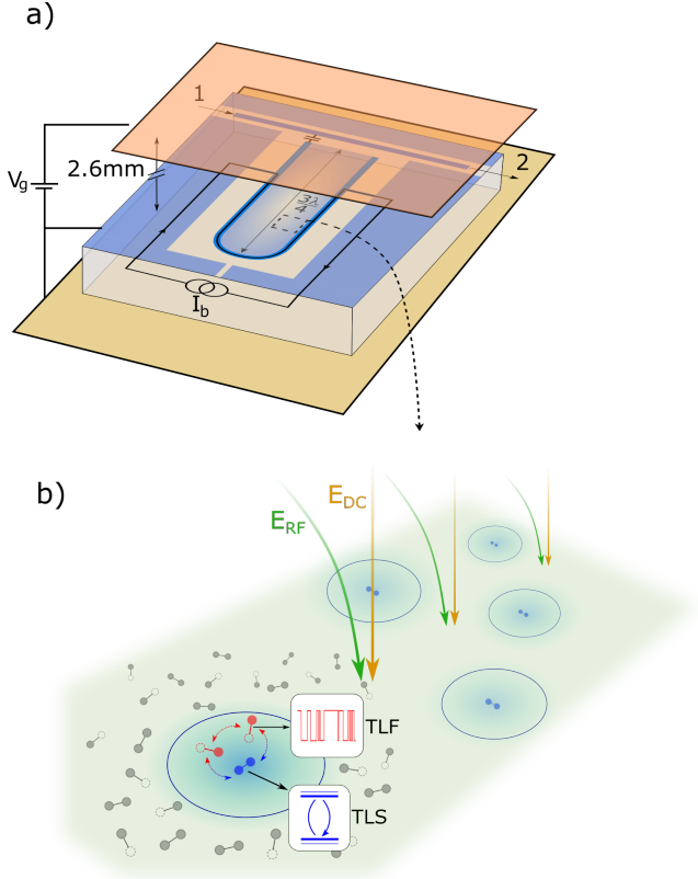
FIG. 1. Planar superconducting resonator as a sensor of fluctuating environmental defects. a) Sketch of the sample setup: tuning resonator frequency (via the applied current I_b ) and external electrostatic gate V_g allow to select individual coherent TLS for study. The resonator is read out by measuring the transmission S_{21} between ports 1 and 2. b) The TLS (blue) couples to a few neighboring incoherent TLFs (red) within the TLS interaction volume (blue circles). The random switching of TLFs causes the telegraph-like fluctuation of TLS excitation energy. The larger bath of background TLFs (grey) affects the TLS linewidth. The TLS couple to the resonator via the microwave electric field E_{RF} , and the DC electric field E_{DC} arising from the applied gate voltage V_g allows to select specific TLS to be in resonance with the resonator.
