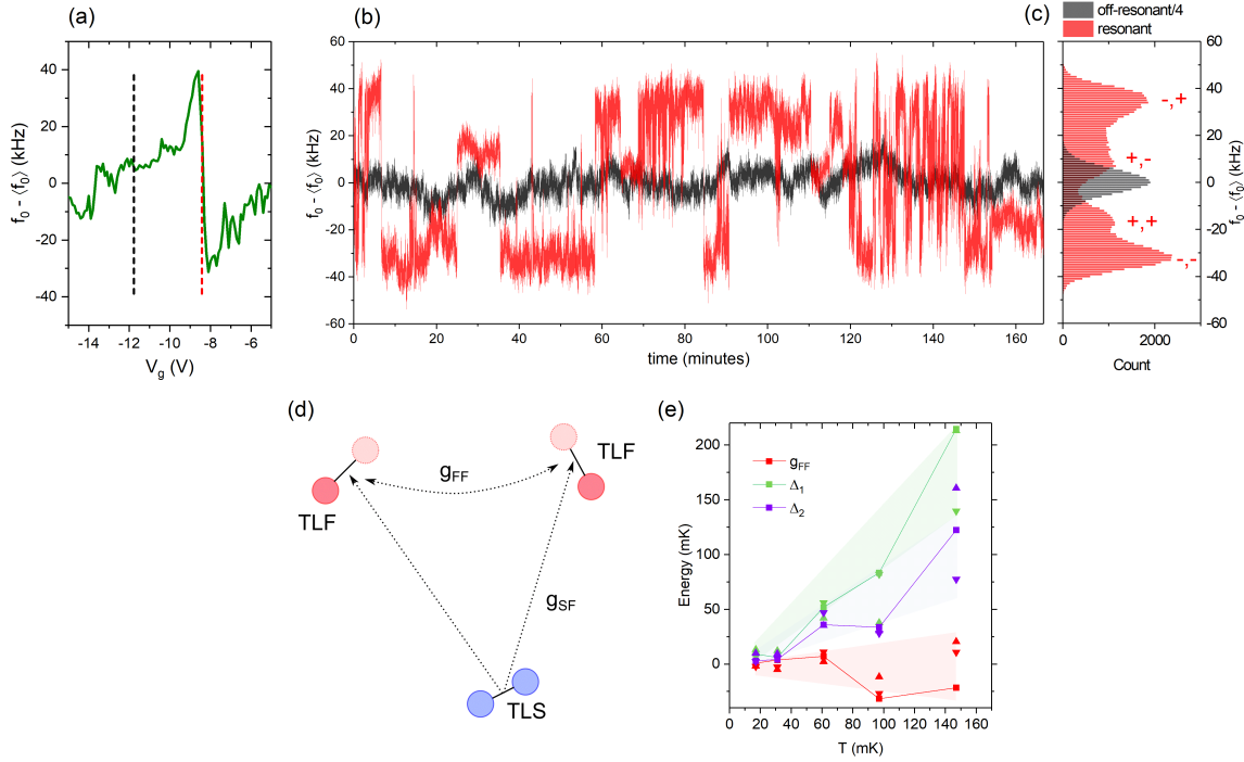
FIG. 3. a) The time-averaged resonator frequency around its resonance with a strongly coupled TLS tuned by the gate. b) Temporal fluctuations of the resonance frequency when resonator and TLS are tuned in (red) and off (black) resonance. Corresponding gate voltages are indicated by the dashed lines in a). The measurements performed at T = 30 mK. c) Histograms of the two time traces in b). d) Sketch of the corresponding microscopic TLF-TLS configuration discussed in the text. g_{FF} and g_{SF} show the couplings between the different entities. e) The fitted TLF energy scales for a range of temperatures.
