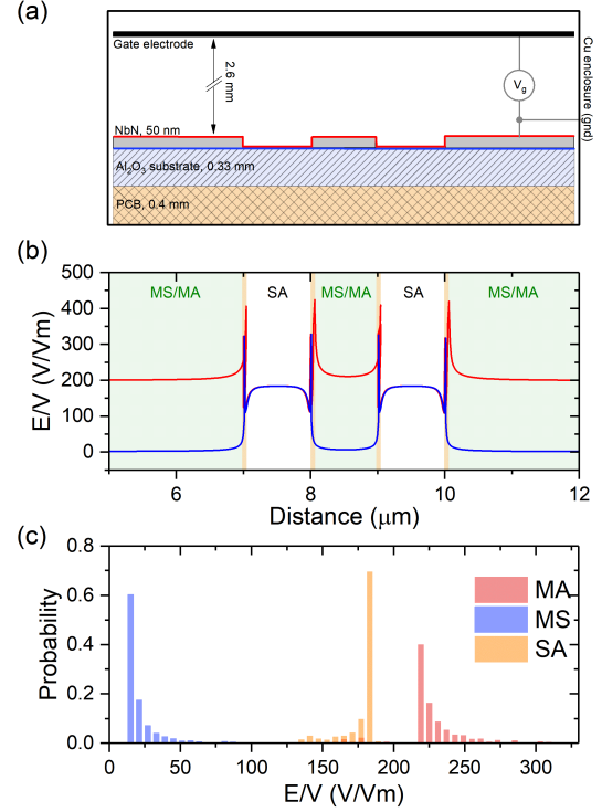
FIG. A1. a) Schematic (not to scale) of the sample and its enclosure outlining the location of the gate electrode and ground potentials with respect to the sample. b) Simulated electric field strength (for 1 V applied to the gate) along the two surfaces indicated by the red and blue contours in a). c) Normalised histogram showing the probability of finding a TLS, randomly placed at the MS or MA interfaces, at a point with a certain electric field strength.
