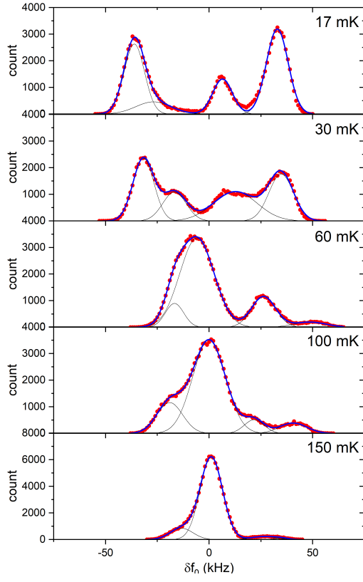
FIG. A3. Distribution of resonator frequency for the coupled resonator-TLS-TLF system together with Gaussian peak fits at different temperatures.
