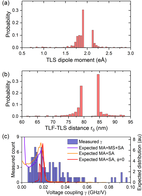
FIG. A2. a) Assuming the TLS is located at either the MA or SA interface we can from the fitted hyperbola and the E-field distribution obtain a probability distribution for the dipole moment of the TLS. b) The probability distribution of the TLF-TLS separation r_0 assuming the rotation angle \phi = 0 . A larger \phi would shift the distribution towards smaller r_0 . c) Measured distribution of TLS voltage coupling coefficients \gamma obtained by fitting a large number of hyperbolas observed across a number of cooldowns. Only hyperbolas that are well defined (e.g. by the TLS minimum energy within or near the measured frequency window) are included in the statistics. The solid lines show the expected distribution obtained from the surface E -field distribution and assuming a uniform angular distribution of TLS orientations.
