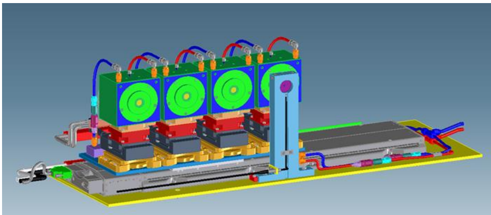
Figure 11: A schematic of the four-wavelength filter radiometer system [reproduced from [29]]
