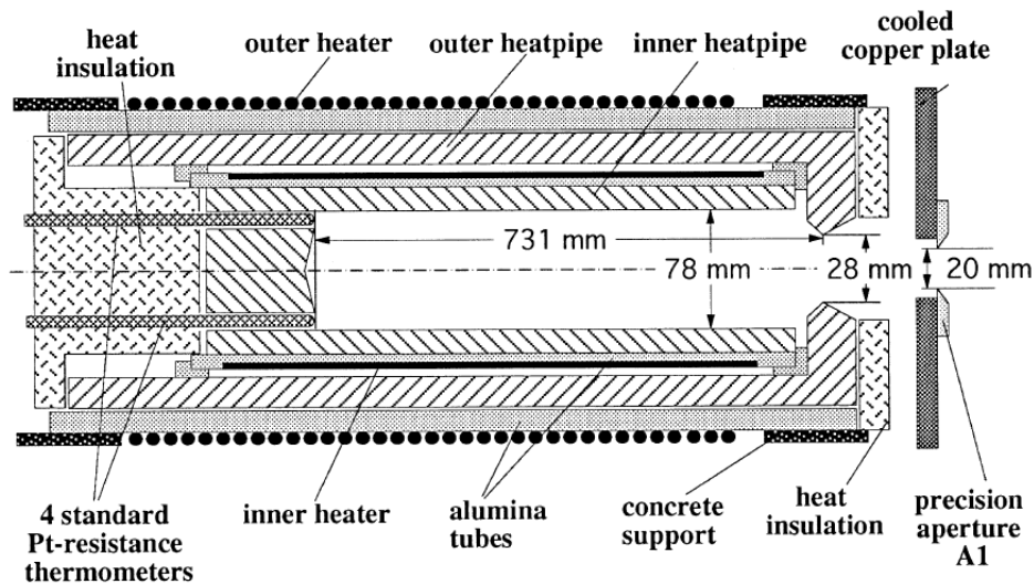
Figure 13: Schematic drawing (not to scale) of the double-heat pipe blackbody [reproduced from [31, 32]]
