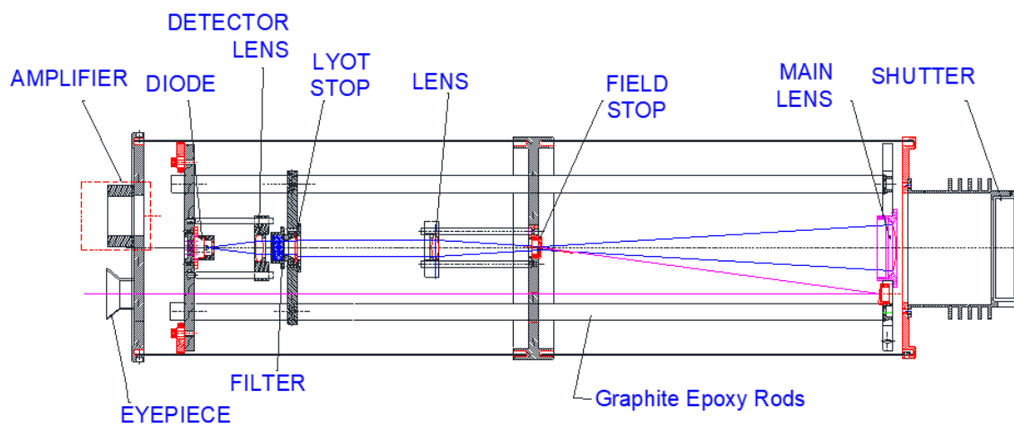
Figure 6: Schematic of the NIST NIRT3 (courtesy of NIST) [reproduced from [18]]
