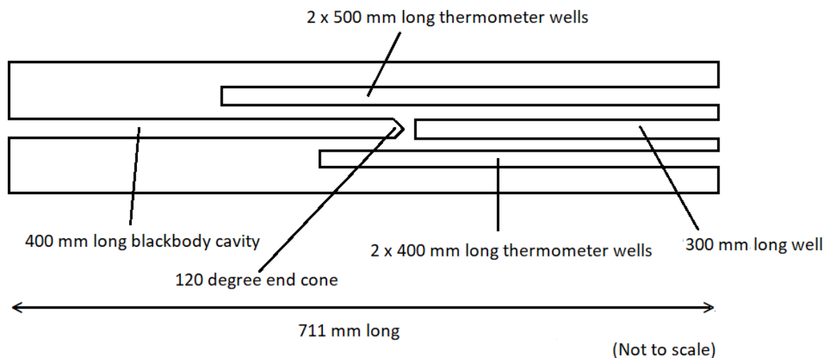
Figure 7: Schematic of one of the PCHPs
