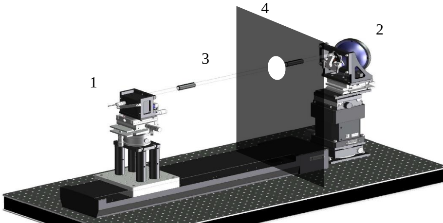
Figure 10: Radiancemeter and monochromatic source of radiance. Trap detector (1), monochromatic source (2), precise gauge (3), baffle (4) [reproduced from [28]]
