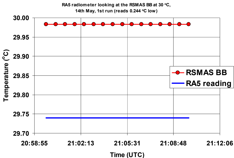
Figure 3.1.28: RA5 radiometer viewing the RSMAS blackbody at 30 °C, 1 st run. \langle \text{Radiometer measurement} \rangle - \text{RSMAS blackbody temperature} = -0.244 \text{ }^{\circ}\text{C} (brackets indicate average over time interval shown).
