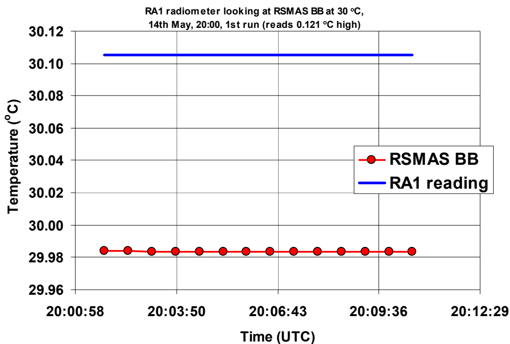
Figure 3.1.4: RA1 radiometer viewing the RSMAS blackbody at 30 °C, 1st measurement. \langle \text{Radiometer measurement} \rangle - \text{RSMAS blackbody temp.} = +0.121 \text{ }^{\circ}\text{C} (brackets indicate average over time interval shown).
