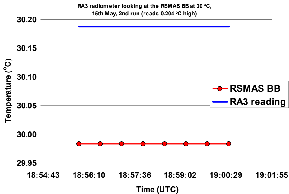
Figure 3.1.17: RA3 radiometer viewing the RSMAS blackbody at 30 °C, 2 nd run. \langle \text{Radiometer measurement} \rangle - \text{RSMAS blackbody temperature} = +0.204 \text{ °C} (brackets indicate average over time interval shown).
