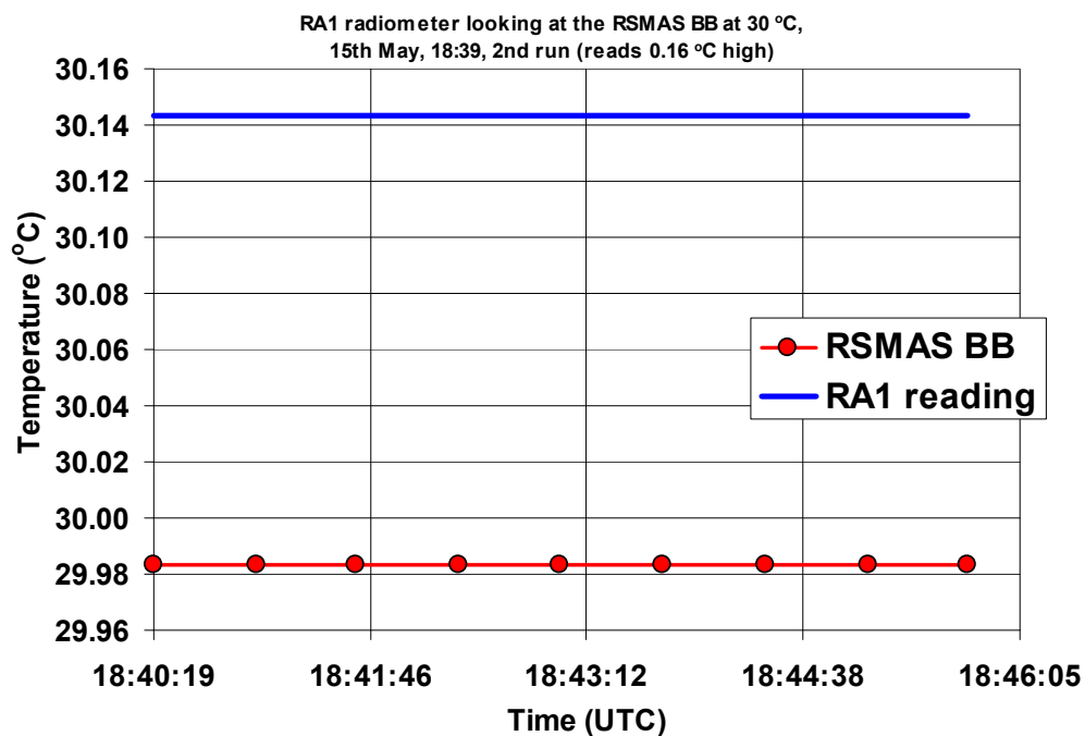
Figure 3.1.5: RA1 radiometer viewing the RSMAS blackbody at 30 °C, 2 nd measurement. \langle \text{Radiometer measurement} \rangle - \text{RSMAS blackbody temp.} = +0.16 \text{ }^{\circ}\text{C} (brackets indicate average over time interval shown).
