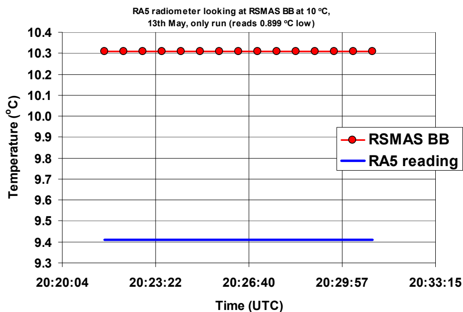
Figure 3.1.25: RA5 radiometer viewing the RSMAS blackbody at 10 °C. \langle \text{Radiometer measurement} \rangle - \text{RSMAS blackbody temperature} = -0.899 \text{ }^{\circ}\text{C} (brackets indicate average over time interval shown).
