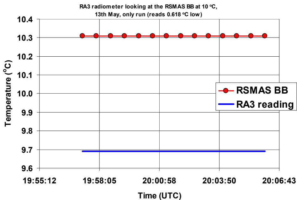
Figure 3.1.13: RA3 radiometer. viewing the RSMAS blackbody at 10 °C. \langle \text{Radiometer measurement} \rangle - \text{RSMAS blackbody temperature} = -0.618\text{ }^{\circ}\text{C} (brackets indicate average over time interval shown).
