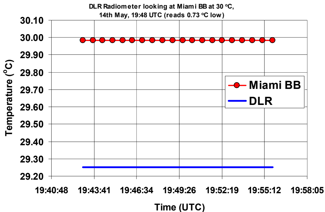
Figure 3.3.5: DLR radiometer viewing the RSMAS blackbody at 30 °C, 1 st run. \langle \text{Radiometer measurement} \rangle - \text{RSMAS blackbody temperature} = -0.73 \text{ }^{\circ}\text{C} (brackets indicate average over time interval shown).
