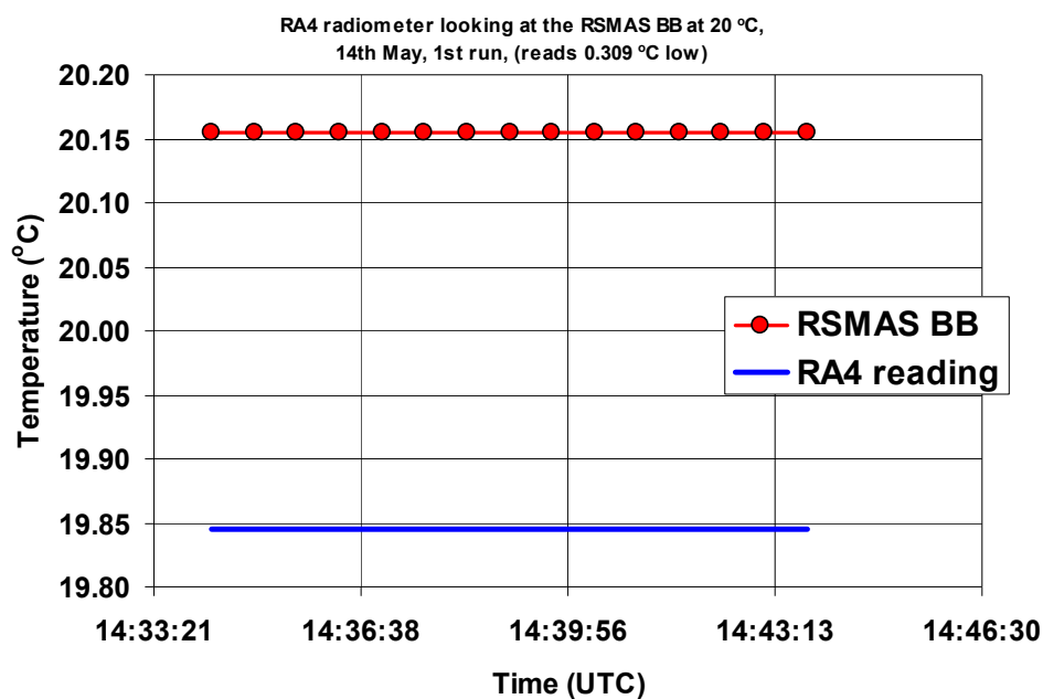
Figure 3.1.20: RA4 radiometer viewing the RSMAS blackbody at 20 °C, 1 st run. \langle \text{Radiometer measurement} \rangle - \text{RSMAS blackbody temperature} = -0.309 \text{ °C} (brackets indicate average over time interval shown).
