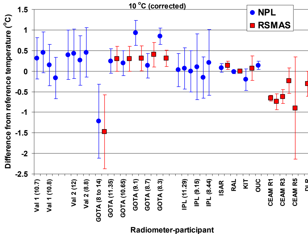
Figure 3.11.4: Plot of the mean of the differences of the radiometer readings from the temperature of the NPL variable temperature blackbody (blue circles), maintained at a nominal temperature of 10 °C. The red squares show the points corresponding to the RSMAS blackbody. This figure corresponds to the corrected values of the IPL radiometer.
