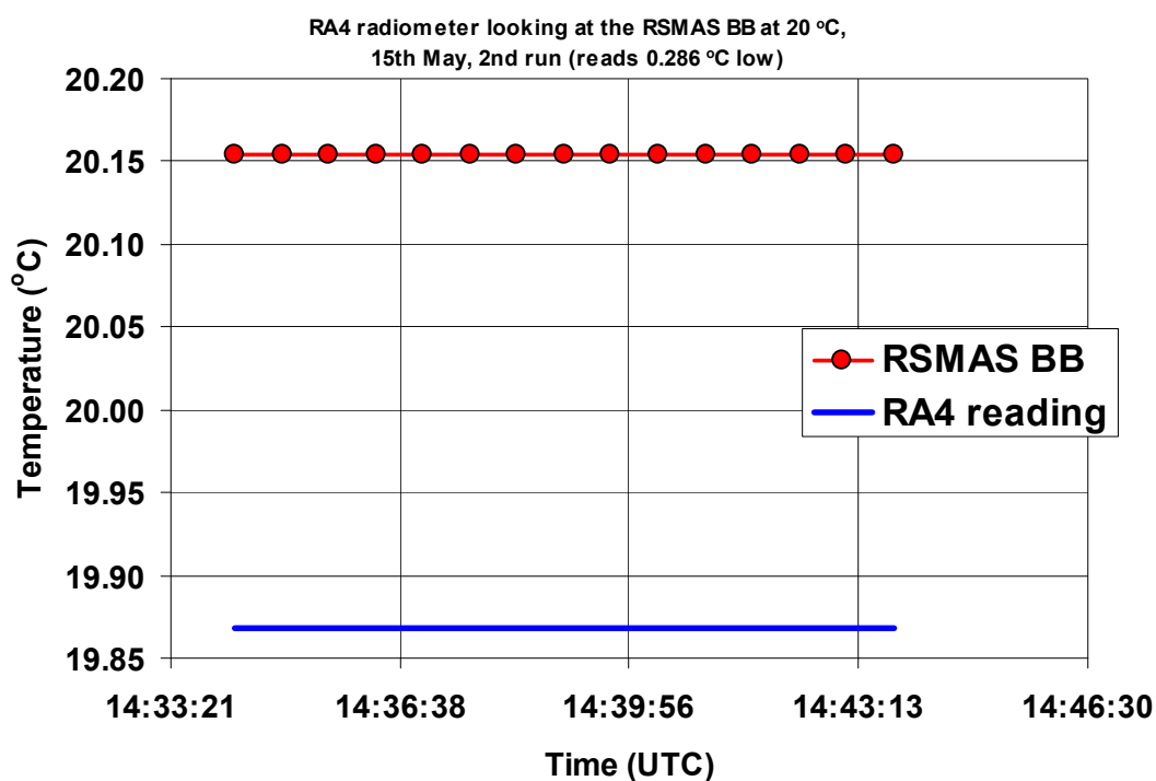
Figure 3.1.21: RA4 radiometer viewing the RSMAS blackbody at 20 °C, 2 nd run. \langle \text{Radiometer measurement} \rangle - \text{RSMAS blackbody temperature} = -0.286 \text{ °C} (brackets indicate average over time interval shown).
