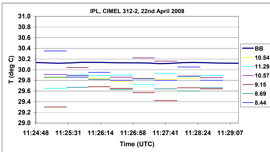
Figure 3.5.10: Plot of the output of the IPL radiometer when it was viewing the NPL blackbody at 30 °C (2nd measurement). The table below this figure lists the deviation of the output of the different radiometer channels \delta T from the average blackbody temperature, over the measurement interval.
