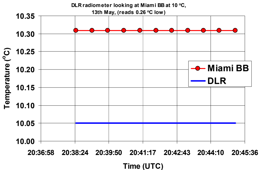
Figure 3.3.2: DLR radiometer viewing the RSMAS blackbody at 10 °C, 2nd run. \langle \text{Radiometer measurement} \rangle - \text{RSMAS blackbody temperature} = -0.26 \text{ }^{\circ}\text{C} (brackets indicate average over time interval shown).
