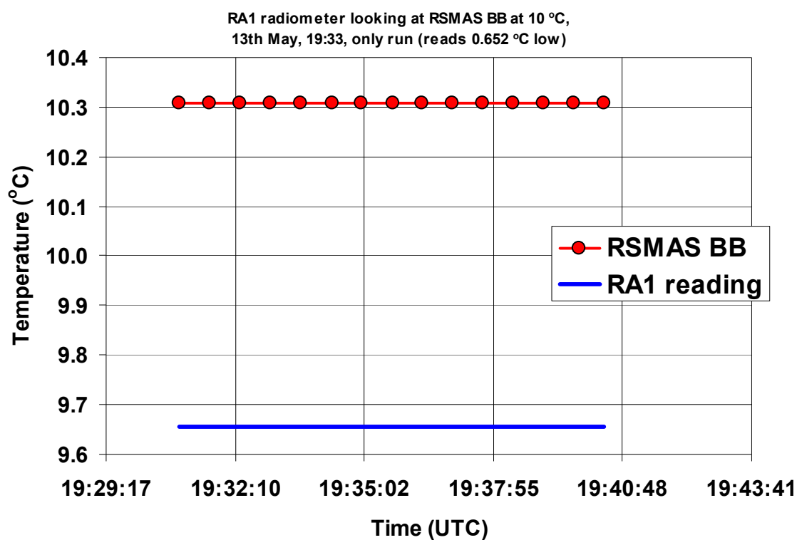
Figure 3.1.1: RA1 radiometer viewing the RSMAS blackbody at 10 °C. \langle \text{Radiometer measurement} \rangle - \text{RSMAS blackbody temperature} = -0.652 \text{ °C} (brackets indicate average over time interval shown).
