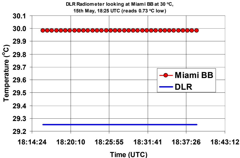
Figure 3.3.6: DLR radiometer viewing the RSMAS blackbody at 30 °C, 2 nd run. \langle \text{Radiometer measurement} \rangle - \text{RSMAS blackbody temperature} = -0.73 \text{ }^{\circ}\text{C} (brackets indicate average over time interval shown).
