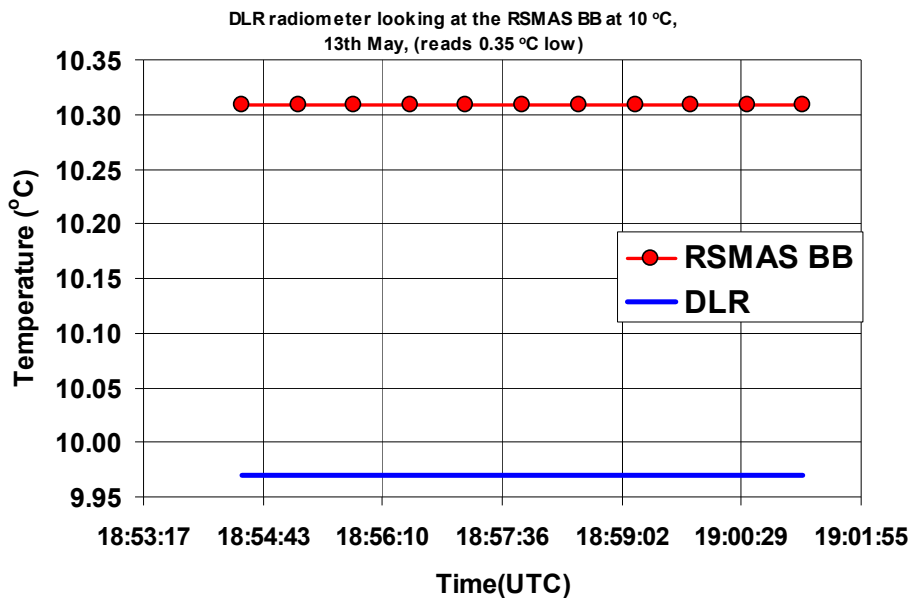
Figure 3.3.1: DLR radiometer viewing the RSMAS blackbody at 10 °C, 1st run. \langle \text{Radiometer measurement} \rangle - \text{RSMAS blackbody temperature} = -0.35 \text{ }^{\circ}\text{C} (brackets indicate average over time interval shown).
