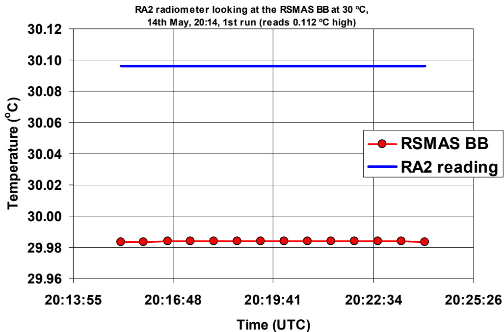
Figure 3.1.10: RA2 radiom. viewing the RSMAS BB at 30 °C, 1 st measurement. \langle \text{Radiometer measurement} \rangle - \text{RSMAS blackbody temperature} = +0.112 \text{ }^{\circ}\text{C} (brackets indicate average over time interval shown).
