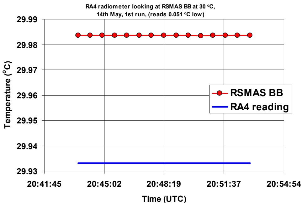
Fig 3.1.22: RA4 radiometer viewing the RSMAS blackbody at 30 °C, 1 st run. \langle \text{Radiometer measurement} \rangle - \text{RSMAS blackbody temperature} = -0.051 \text{ }^{\circ}\text{C} (brackets indicate average over time interval shown).
