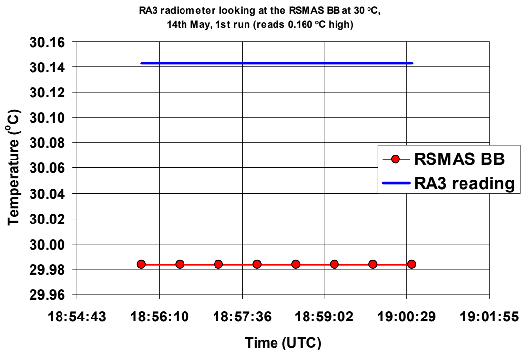
Figure 3.1.16: RA3 radiometer viewing the RSMAS blackbody at 30 °C, 1 st run. \langle \text{Radiometer measurement} \rangle - \text{RSMAS blackbody temperature} = +0.16 \text{ °C} (brackets indicate average over time interval shown).
