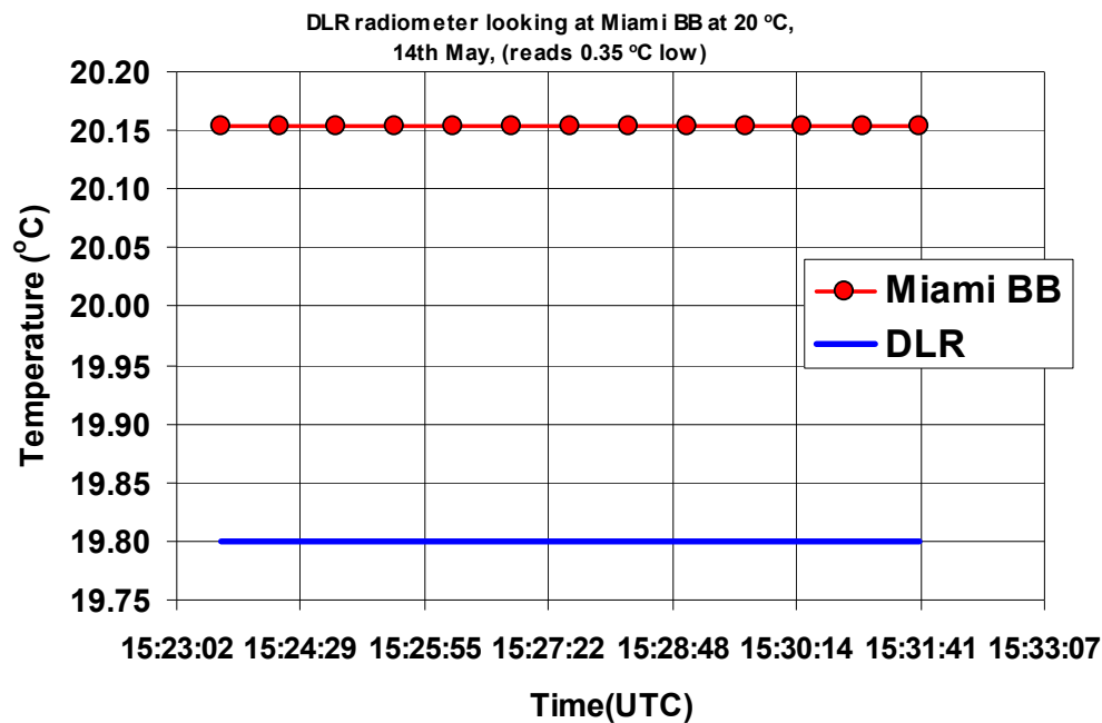
Figure 3.3.3: DLR radiometer viewing the RSMAS blackbody at 20 °C, 1 st run. \langle \text{Radiometer measurement} \rangle - \text{RSMAS blackbody temperature} = -0.35 \text{ }^{\circ}\text{C} (brackets indicate average over time interval shown).
