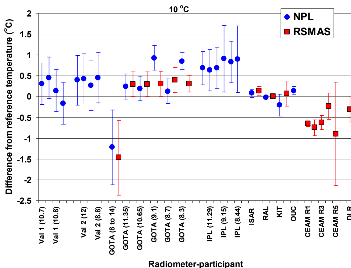
Figure 3.11.3: Plot of the mean of the differences of the radiometer readings from the temperature of the NPL variable temperature blackbody (blue circles), maintained at a nominal temperature of 10 °C. The red squares show the points corresponding to the RSMAS blackbody. This figure corresponds to the uncorrected values of the IPL radiometer.
