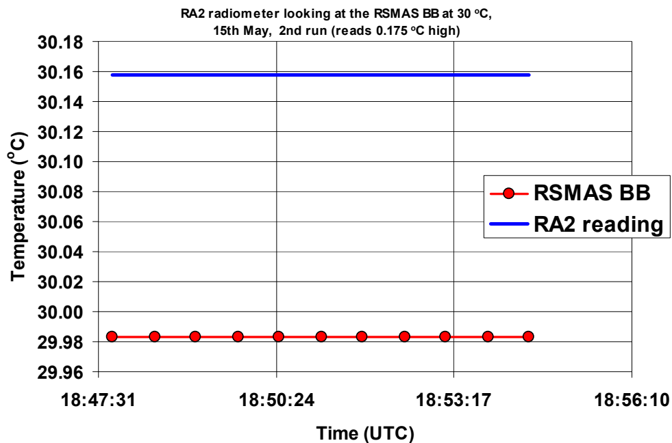
Figure 3.1.11: RA2 radiom. viewing the RSMAS BB at 30 °C, 2 nd measurement. \langle \text{Radiometer measurement} \rangle - \text{RSMAS blackbody temperature} = +0.175 \text{ }^{\circ}\text{C} (brackets indicate average over time interval shown).
