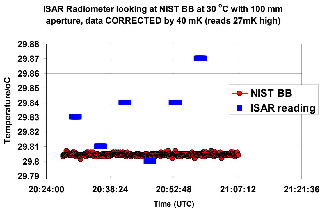
Figure 3.7.14: ISAR radiometer viewing the NIST blackbody at 30 °C, 100 mm aperture, \langle \text{Radiometer measurement} \rangle - \text{NIST blackbody temp} = 0.027 \text{ K} , (brackets indicate average over time interval shown)
