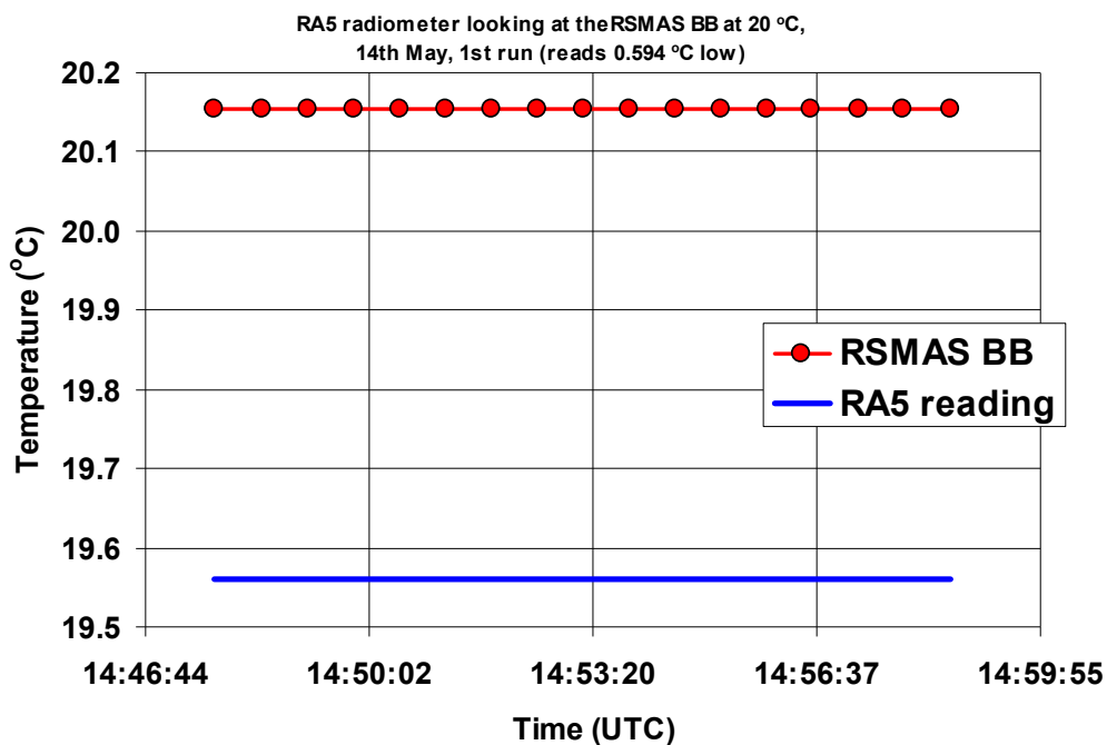
Figure 3.1.26: RA5 radiometer viewing the RSMAS blackbody at 20 °C, 1 st run. \langle \text{Radiometer measurement} \rangle - \text{RSMAS blackbody temperature} = -0.594 \text{ °C} (brackets indicate average over time interval shown).
