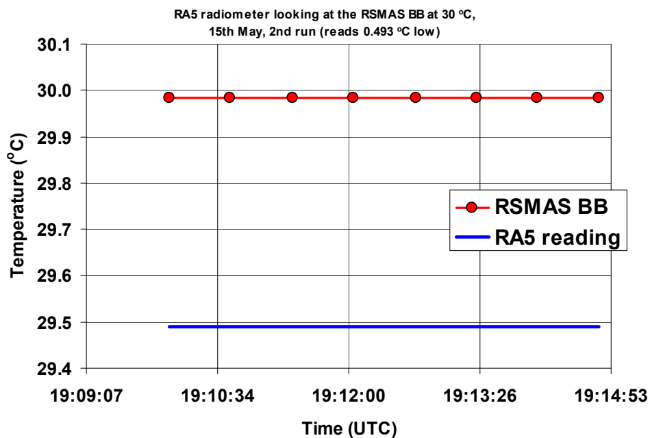
Figure 3.1.29: RA5 radiometer viewing the RSMAS blackbody at 30 °C, 2 nd run. \langle \text{Radiometer measurement} \rangle - \text{RSMAS blackbody temperature} = -0.493 \text{ }^{\circ}\text{C} (brackets indicate average over time interval shown).
