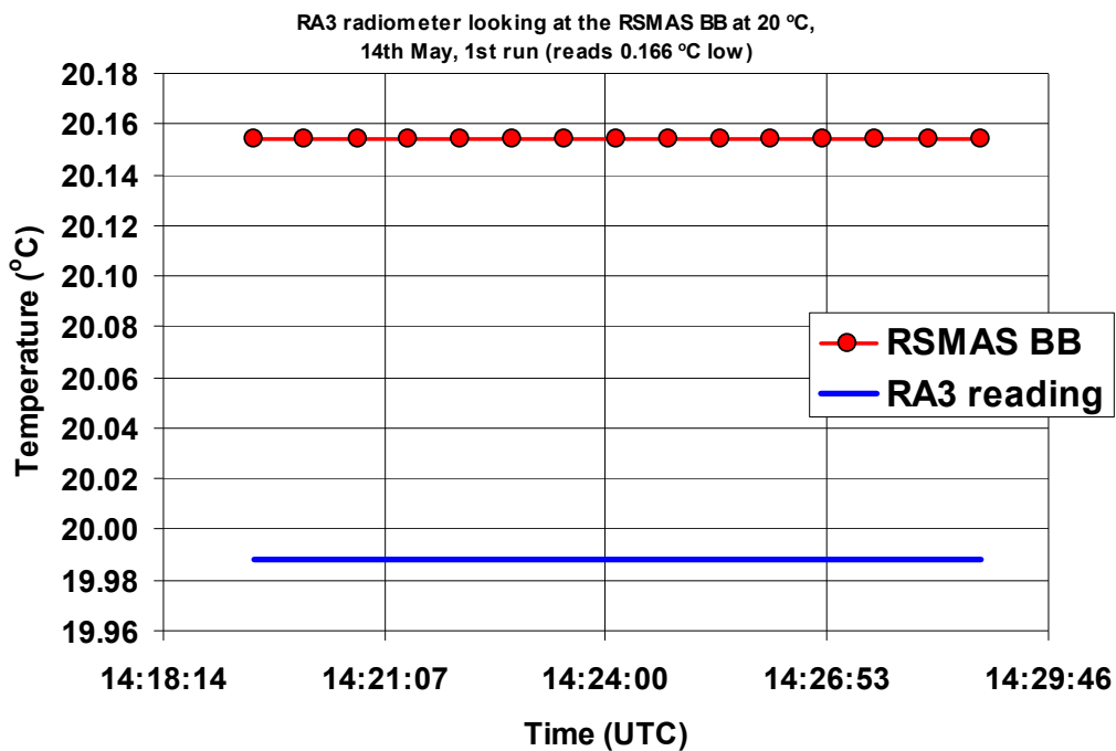
Figure 3.1.14: RA3 radiometer viewing the RSMAS blackbody at 20 °C, 1 st run. \langle \text{Radiometer measurement} \rangle - \text{RSMAS blackbody temperature} = -0.166 \text{ °C} (brackets indicate average over time interval shown).
