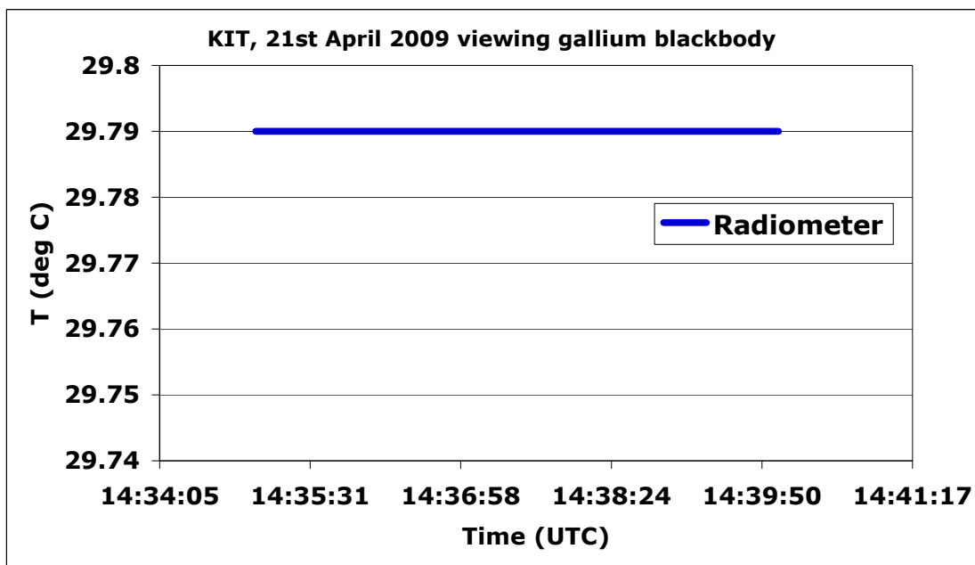
Fig 3.6.6: KIT ground radiometer viewing the NPL gallium blackbody. Radiometer measurement - Gallium melting temp. = 0.025 K (brackets indicate average over time interval shown)
