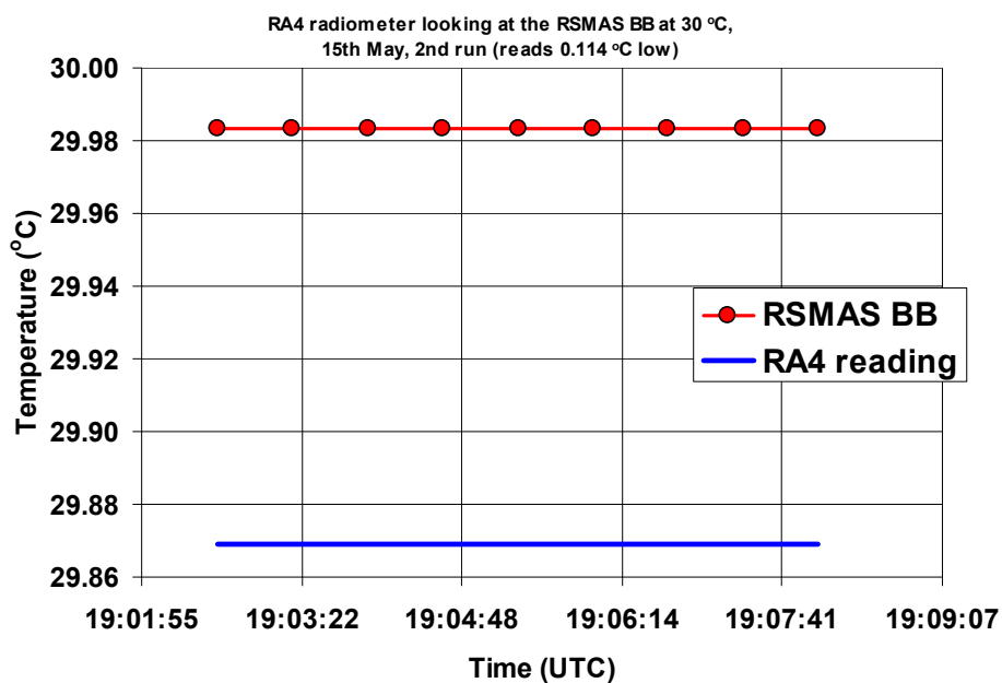
Figure 3.1.23: RA4 radiometer viewing the RSMAS blackbody at 30 °C. \langle \text{Radiometer measurement} \rangle - \text{RSMAS blackbody temperature} = -0.114 \text{ }^{\circ}\text{C} (brackets indicate average over time interval shown).
