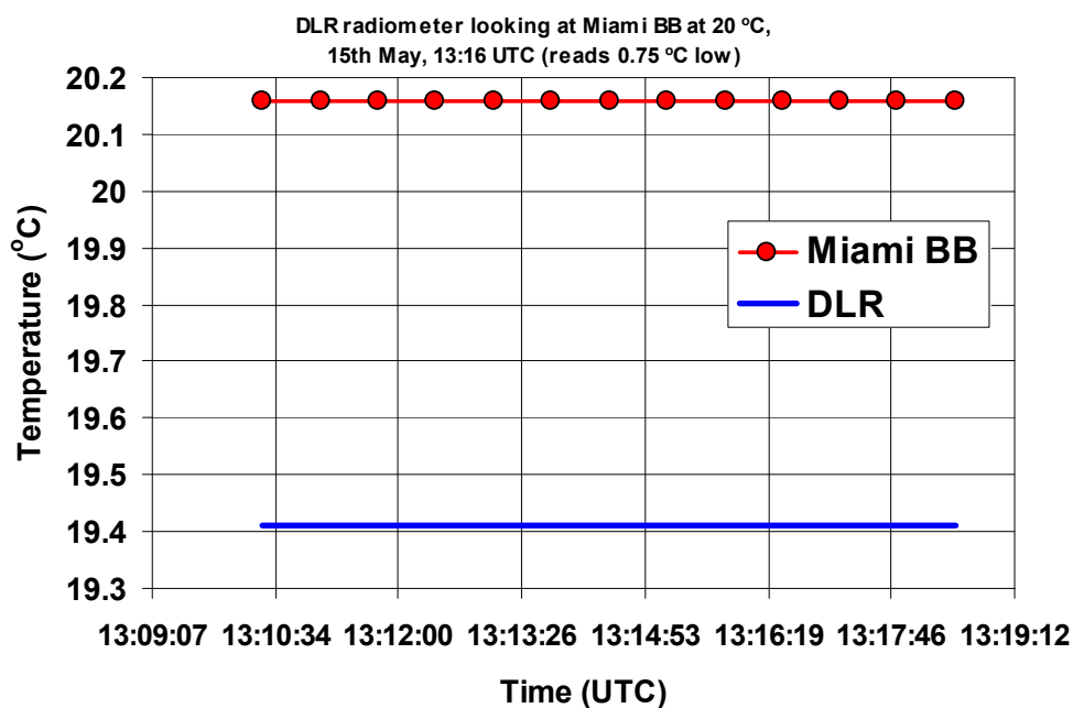
Figure 3.3.4: DLR radiometer viewing the RSMAS blackbody at 20 °C, 2nd run. \langle \text{Radiometer measurement} \rangle - \text{RSMAS blackbody temperature} = -0.75 \text{ }^{\circ}\text{C} (brackets indicate average over time interval shown).
