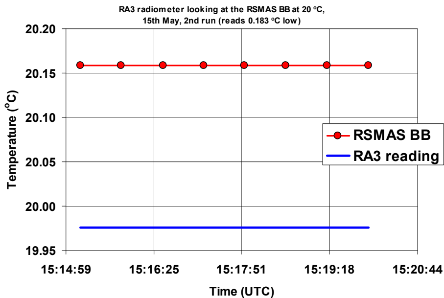
Figure 3.1.15: RA3 radiometer viewing the RSMAS blackbody at 20 °C, 2 nd run. \langle \text{Radiometer measurement} \rangle - \text{RSMAS blackbody temperature} = -0.183 \text{ °C} (brackets indicate average over time interval shown).
