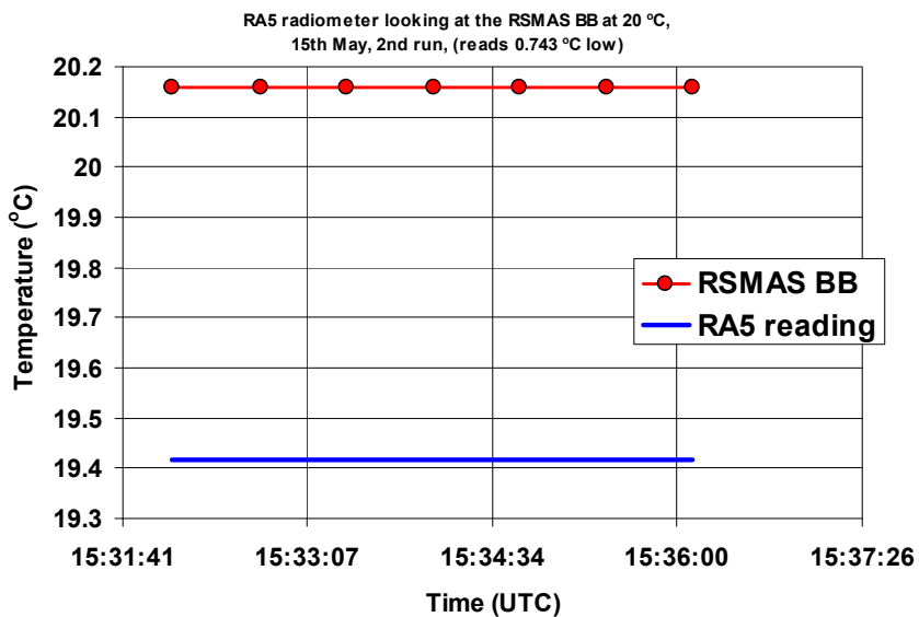
Figure 3.1.27: RA5 radiometer viewing the RSMAS blackbody at 20 °C, 2 nd run. \langle \text{Radiometer measurement} \rangle - \text{RSMAS blackbody temperature} = -0.743 \text{ °C} (brackets indicate average over time interval shown).
