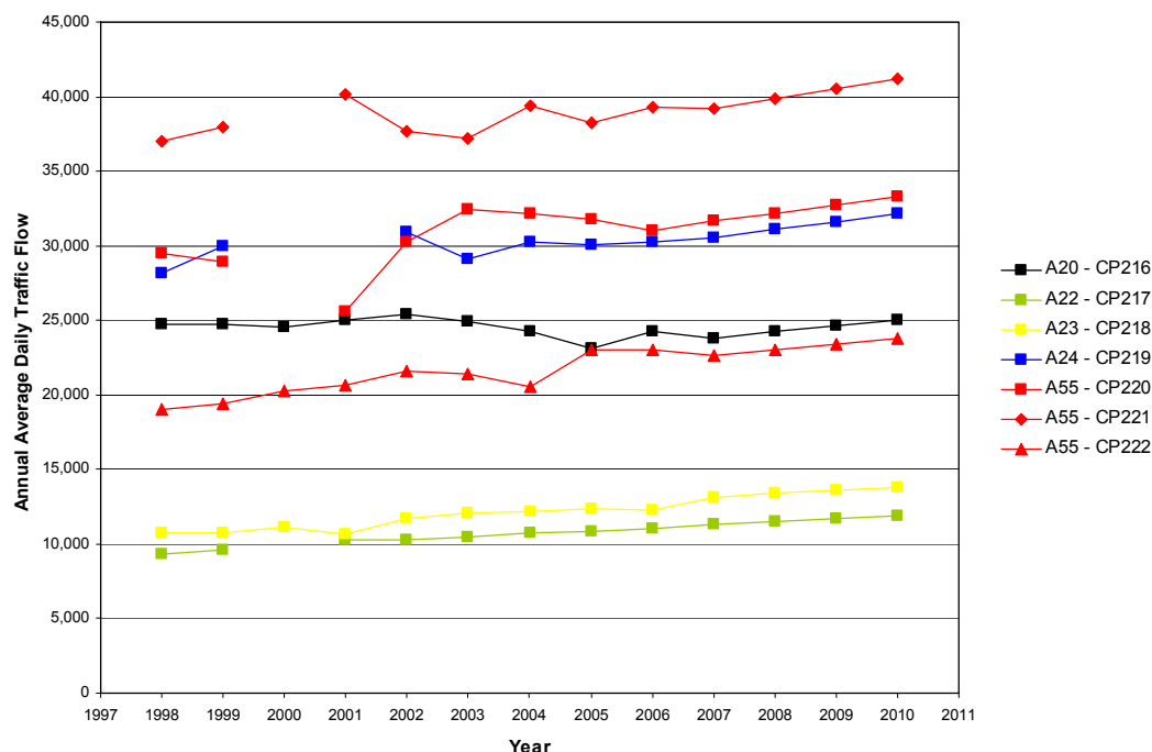
Figure 3-3: Time series of actual and forecast traffic counts (7-day AADT) at traffic census points in and around Castlereagh Borough.
