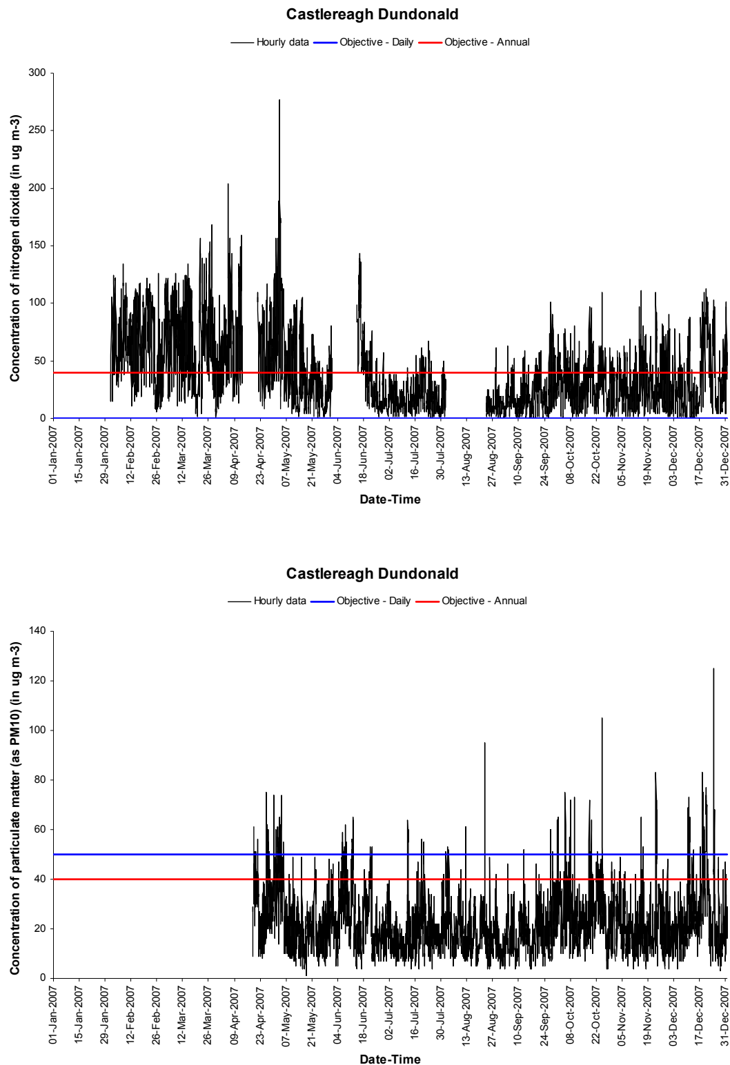
Figure A1.3: 2007 hourly measurements of nitrogen dioxide (in \mu\text{g NO}_2 \text{ m}^{-3} , upper panel) and of particulate matter (as \text{PM}_{10} in \mu\text{g m}^{-3} , lower panel) for the Castlereagh Dundonald site.
