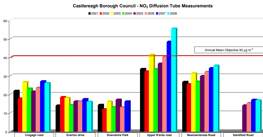
Figure 2-3: Trends in the measured annual mean NO 2 concentrations (in \mu\text{g}/\text{m}^3 ) at diffusion tube sites in Castlereagh.
