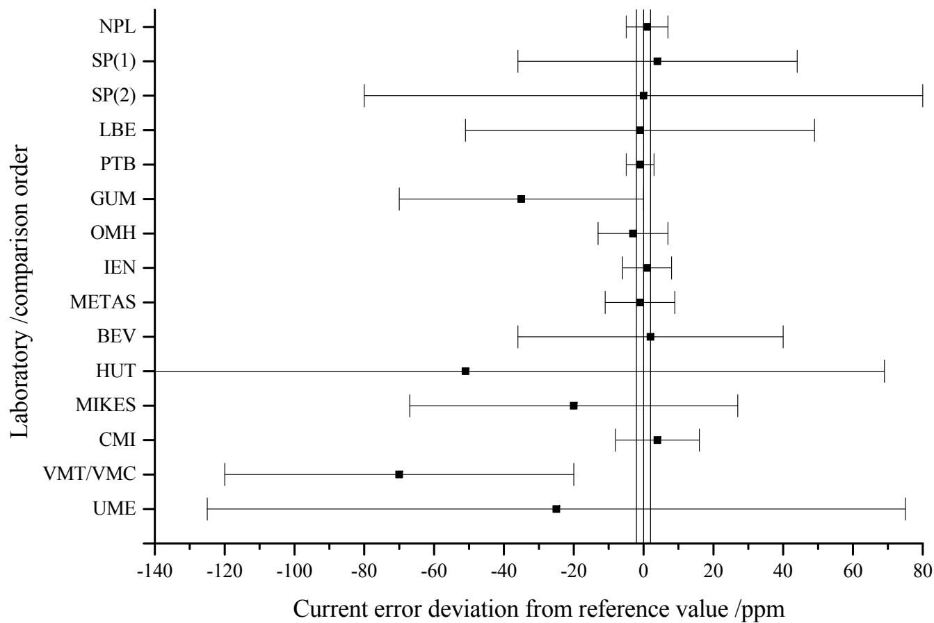
Figure 13: Ratio 500 / 5, I/I_n = 100\% , current error comparison results
