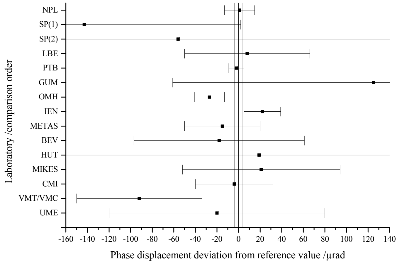
Figure 16: Ratio 500 / 5, I/I_n = 2\% , phase displacement comparison results
