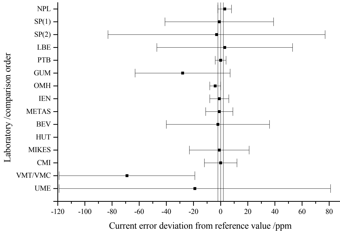
Figure 8: Ratio 10 / 5, I/I_n = 100\% , current error comparison results
