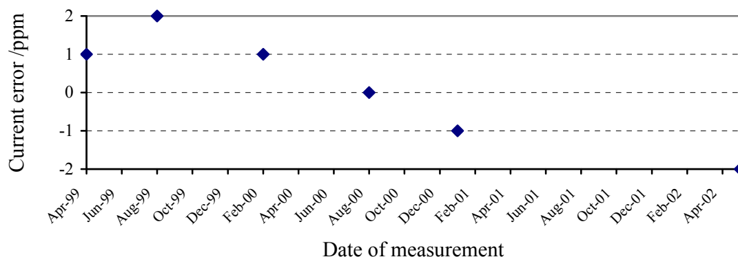
Figure 1: Ratio 50 / 5, I/I_n = 100\% , Transfer standard behaviour
