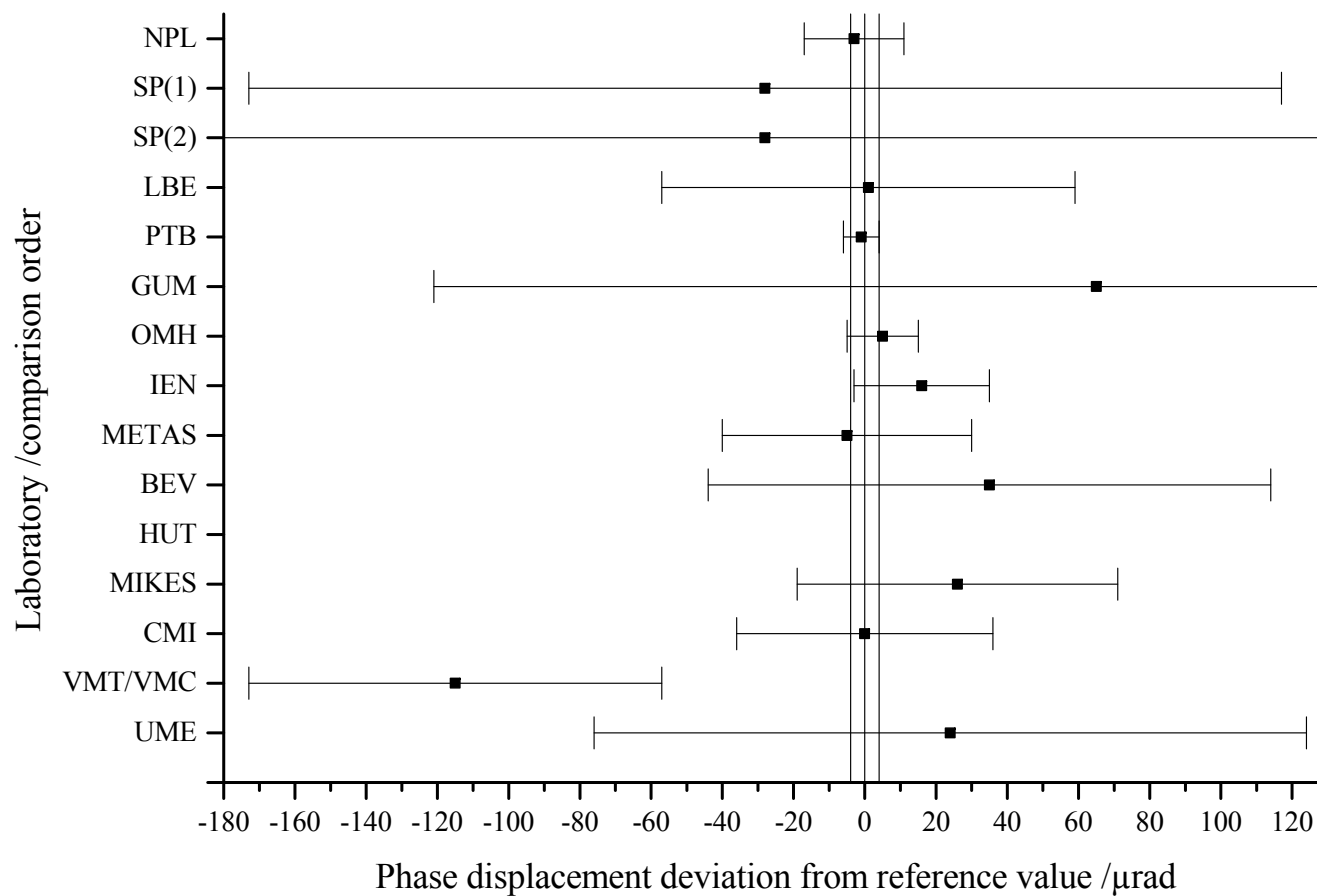
Figure 7: Ratio 5 / 5, I/I_n = 2\% , phase displacement comparison results
