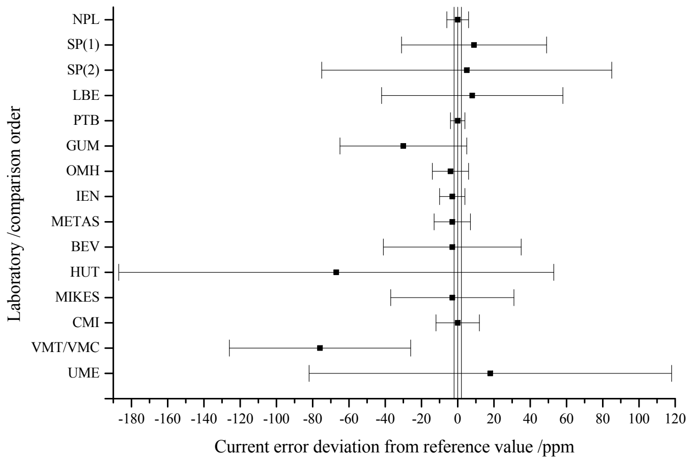
Figure 11: Ratio 100 / 5, I/I_n = 100\% , current error comparison results
