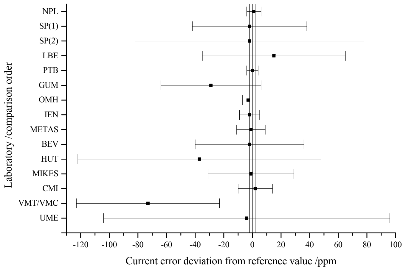
Figure 9: Ratio 20 / 5, I/I_n = 100\% , current error comparison results
