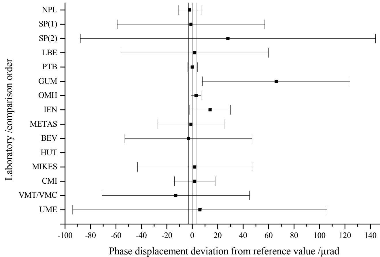
Figure 6: Ratio 5 / 5, I/I_n = 100\% , phase displacement comparison results
