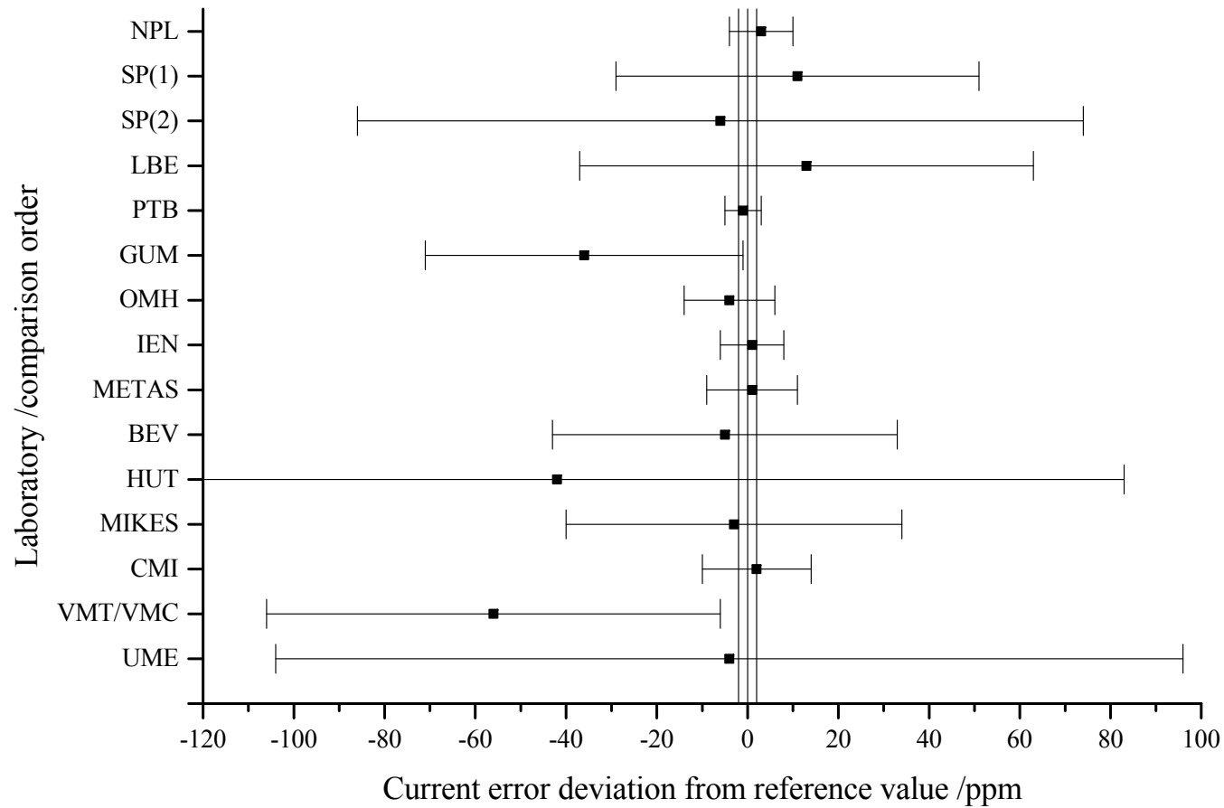
Figure 12: Ratio 200 / 5, I/I_n = 100\% , current error comparison results
