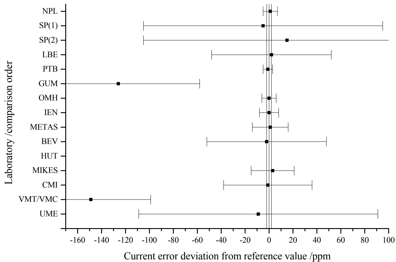
Figure 5: Ratio 5 / 5, I/I_n = 2\% , current error comparison results
