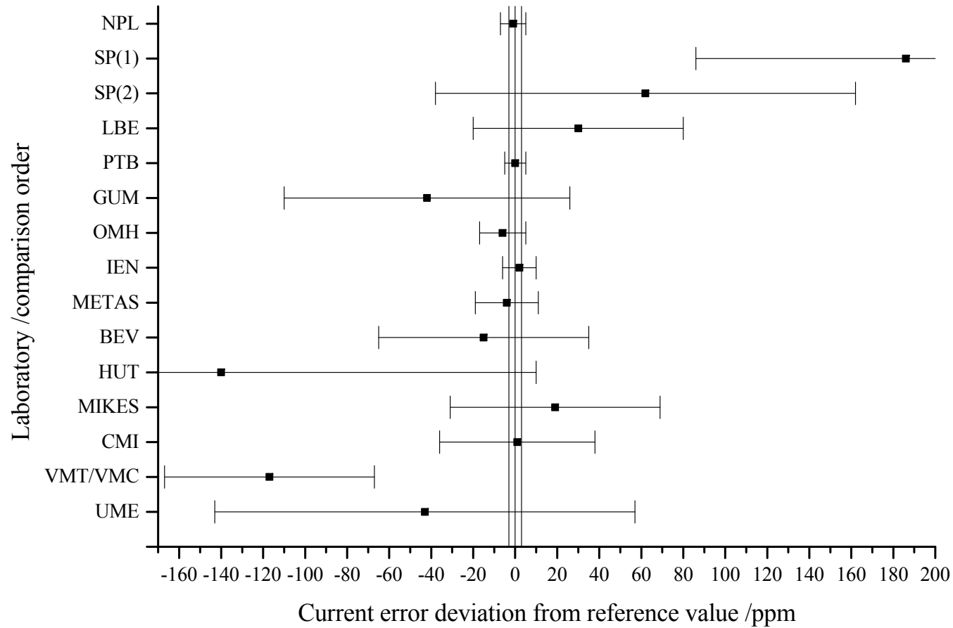
Figure 14: Ratio 500 / 5, I/I_n = 2\% , current error comparison results
