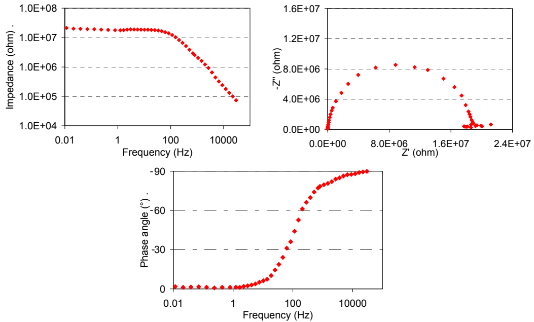
Figure 8. Impedance results for Cu board
