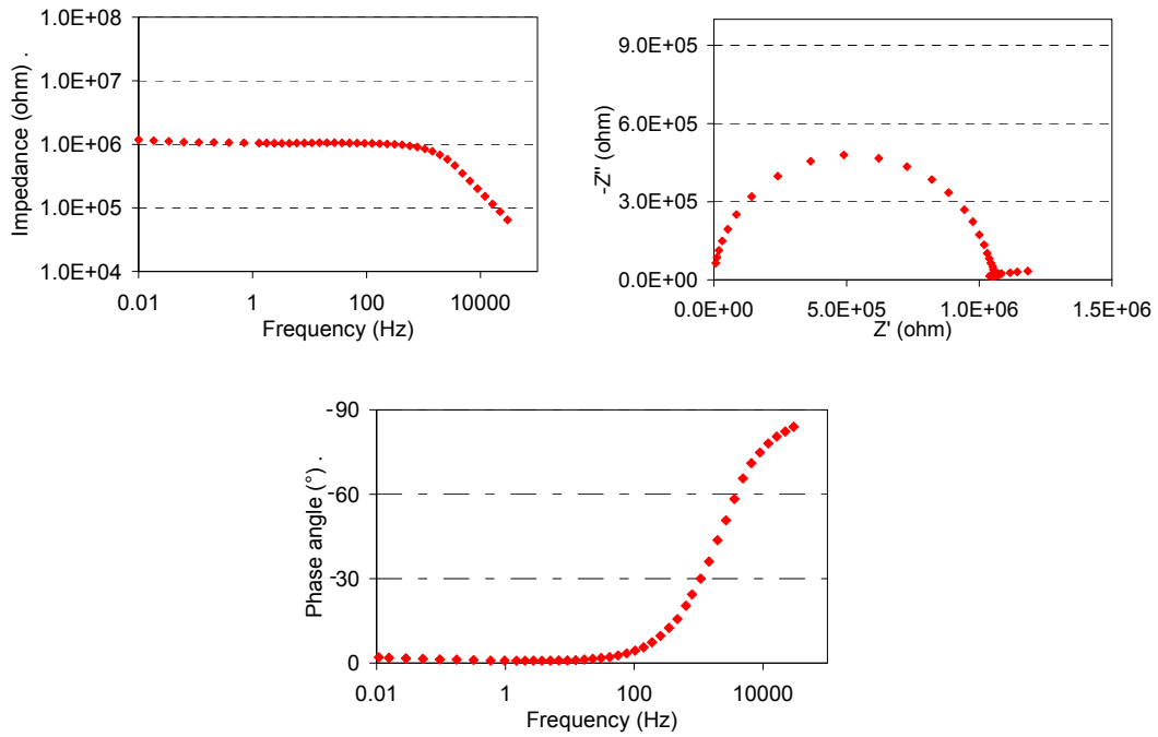
Figure 7. Impedance results for Sn board
