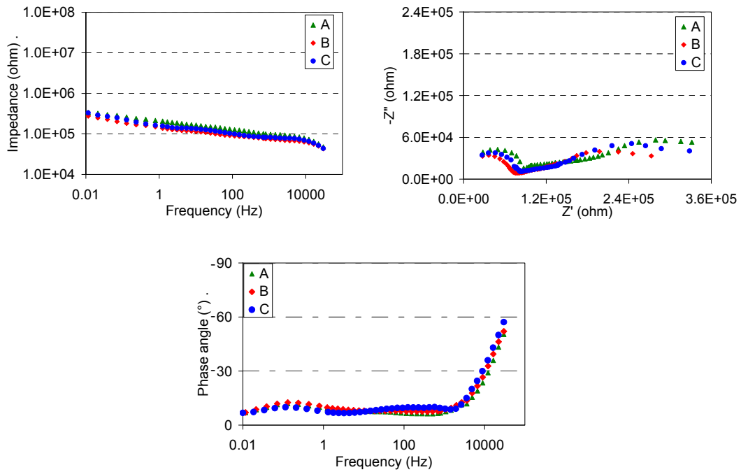
Figure 4. Impedance results for ENIG board
