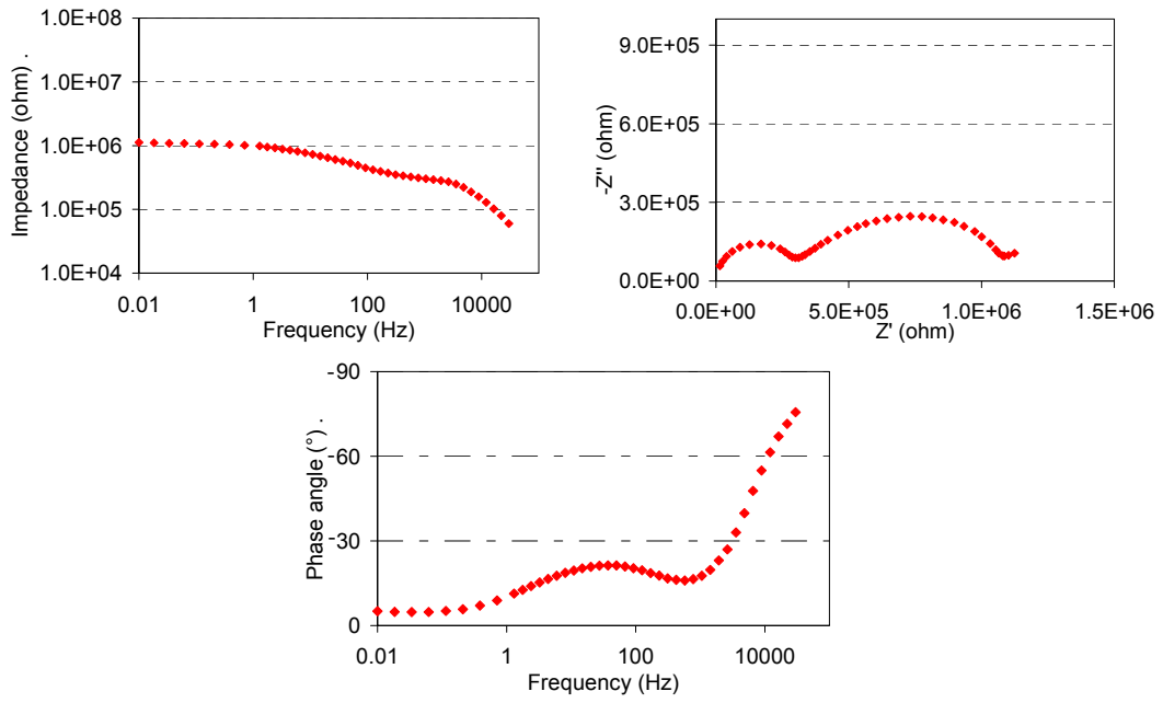
Figure 5. Impedance results for SnPb board
