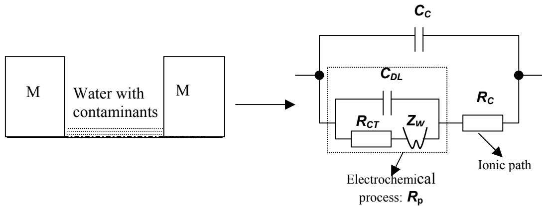
Figure 1. Conduction path for conductor-insulator structure
