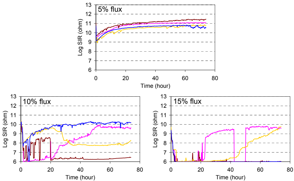
Figure 10. SIR results from ENIG boards with three concentrations of flux
