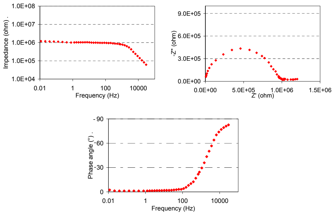
Figure 6. Impedance results for SAC board
