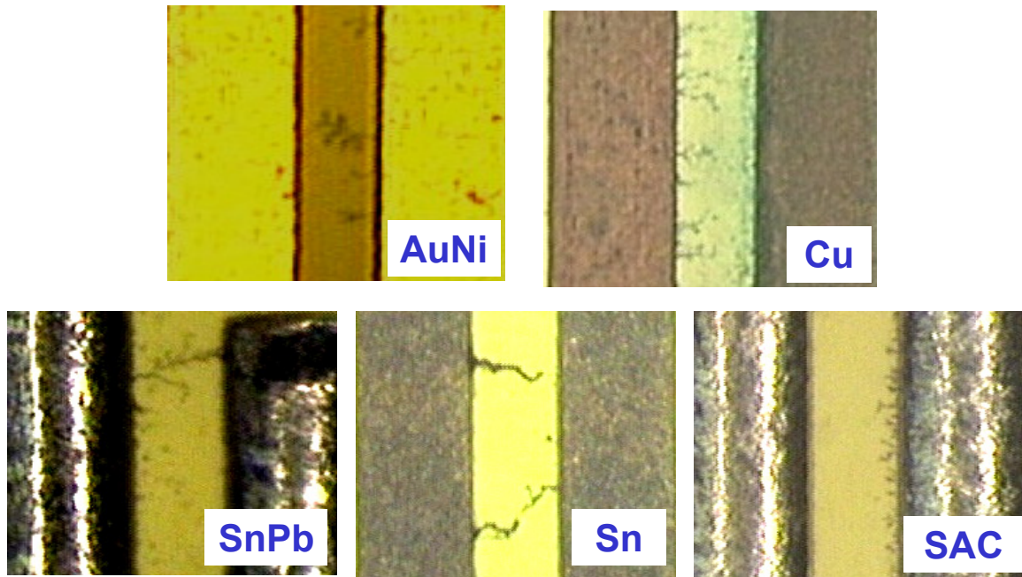
Figure 16. Dendrites formed on different board finish
