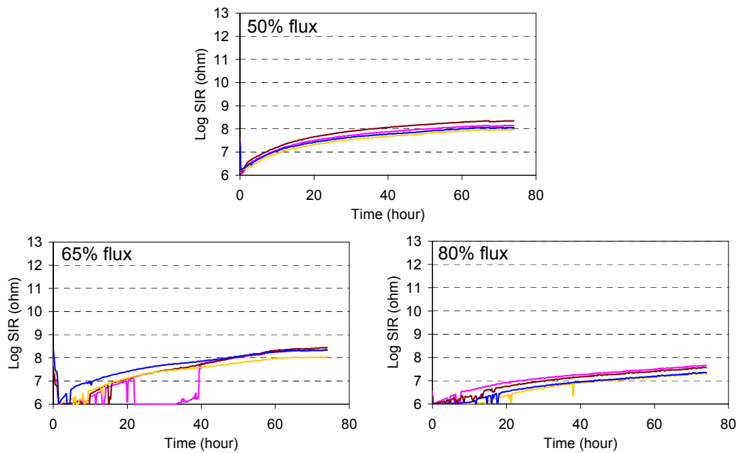
Figure 14. SIR results from Cu boards with three concentrations of flux
