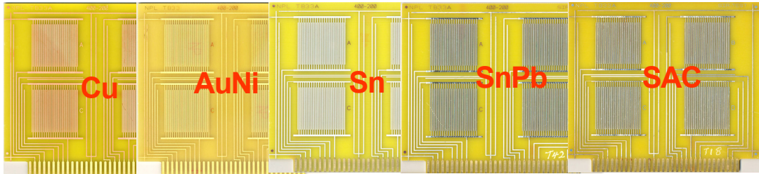
Figure 2. Test board with five finishes
