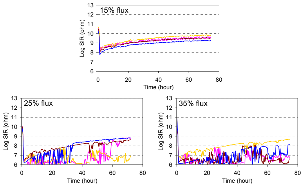
Figure 13. SIR results from Sn boards with three concentrations of flux
