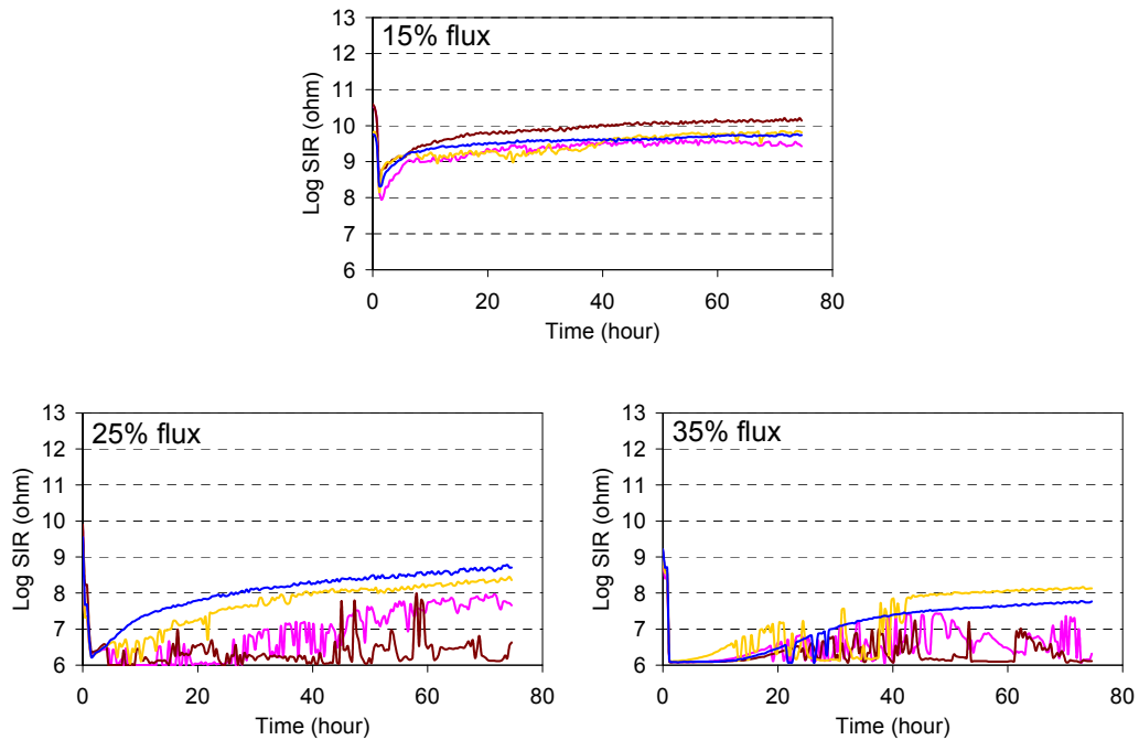
Figure 12. SIR results from SAC boards with three concentrations of flux
