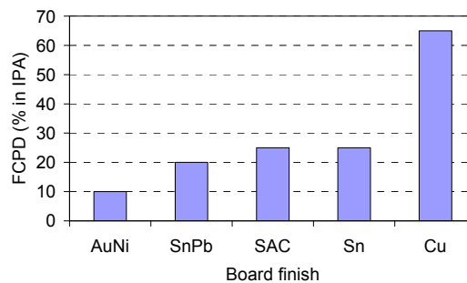
Figure 15. The FCPD on different board finishes
