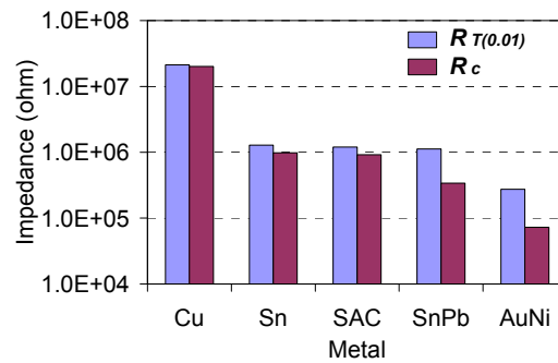
Figure 9. R_{T(0.01)} and R_c for five board finishes
