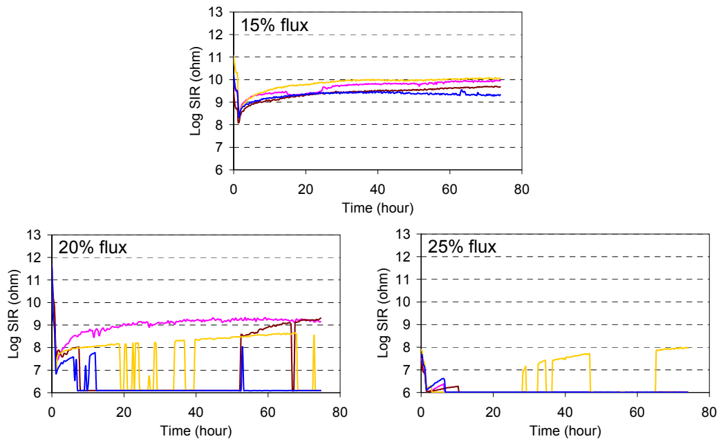
Figure 11. SIR results from SnPb boards with three concentrations of flux
