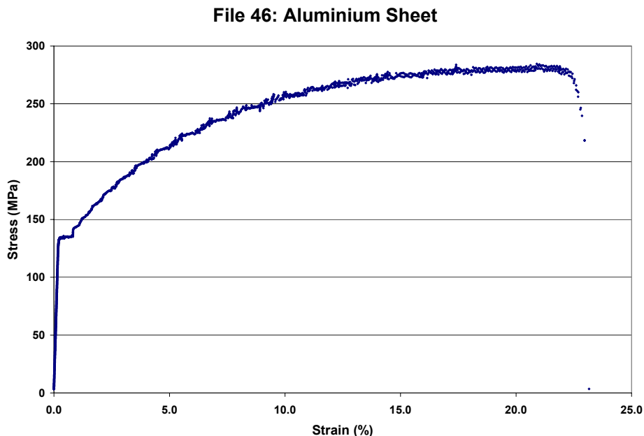
Fig 21: Stress-strain curve showing serrated yielding.
