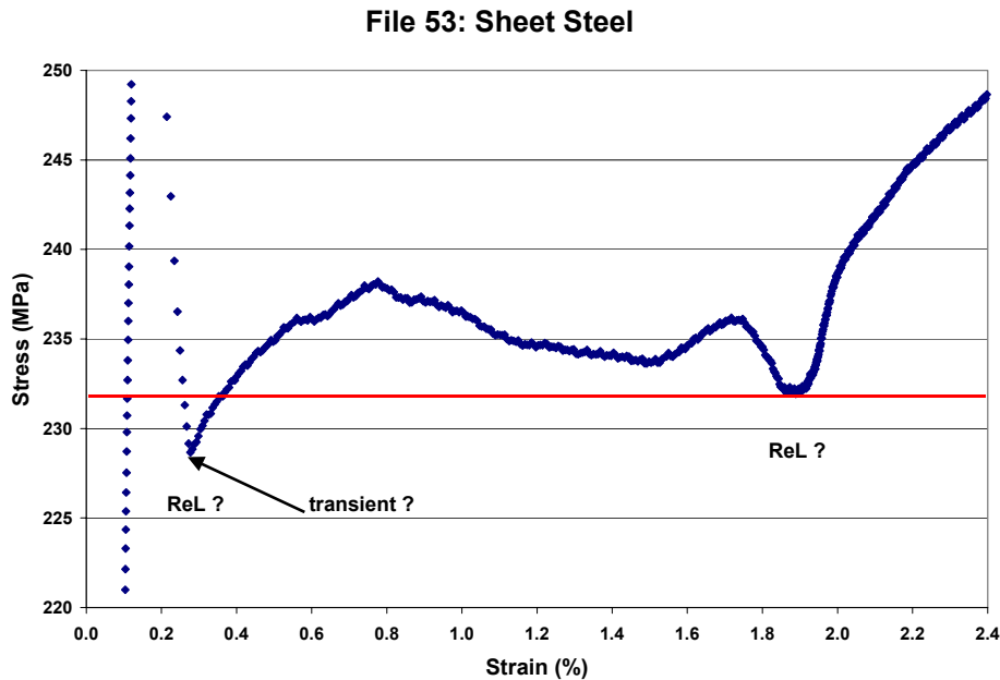
Fig 13: Transient effects and the impact on the selection of R_{eL} (File 53)
