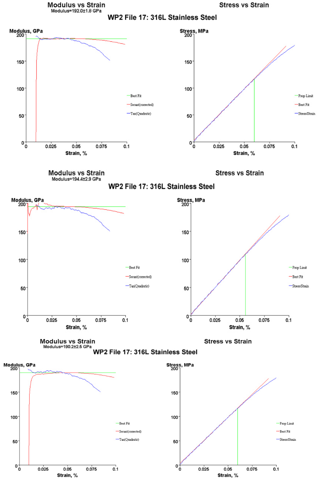
Fig 8: Examples showing the sensitivity of the tangent/secant approach
