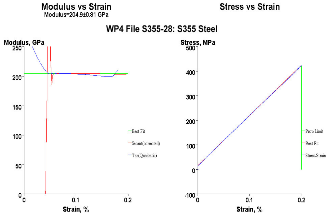
Fig 19: Analysis of NPL WP4 stress-strain curve for the S355 material (File S355-28) - Test Conditions 2.1
