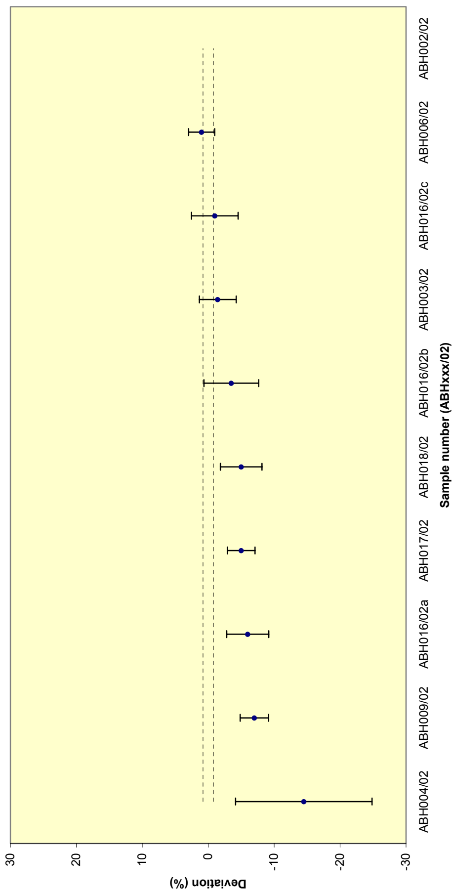
Figure 19 - Reported ^{238}\text{Pu} results (high level) (one outside limit of plot)
