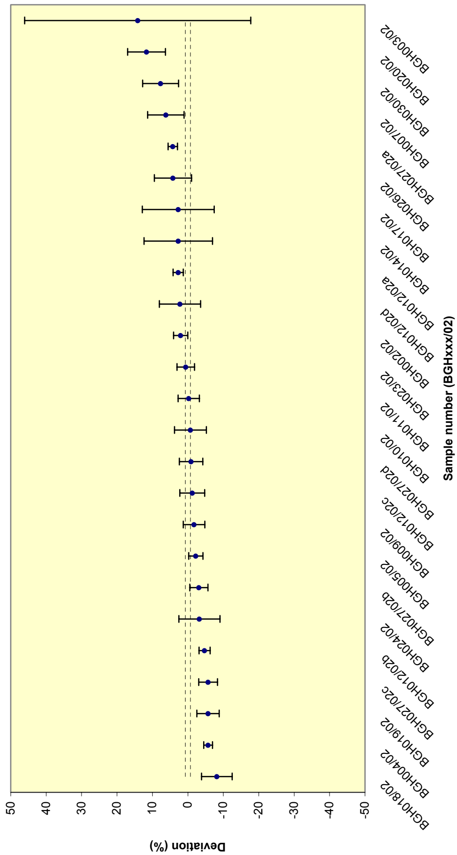
Figure 67 - Reported ^{137}\text{Cs} results (high level)
