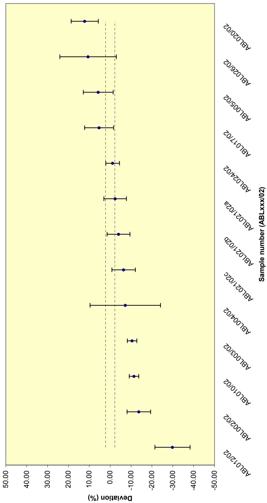
Figure 1 - Reported ^{90}\text{Sr} results (low level)
