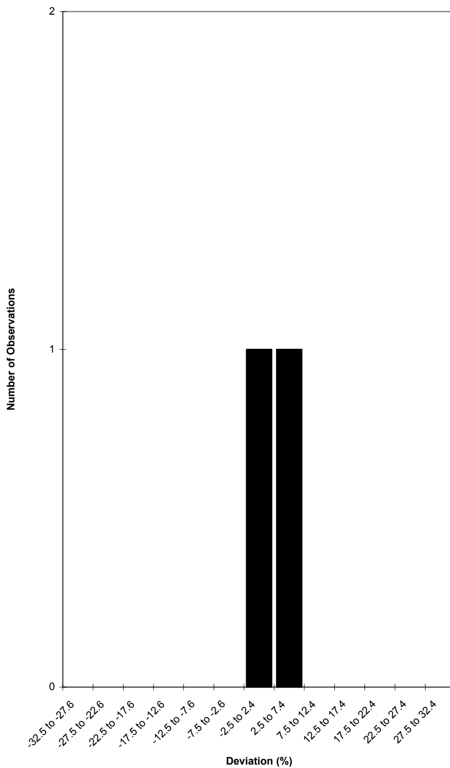
Figure 36 ^{35}\text{S} High level results (One outside limits of plot)
