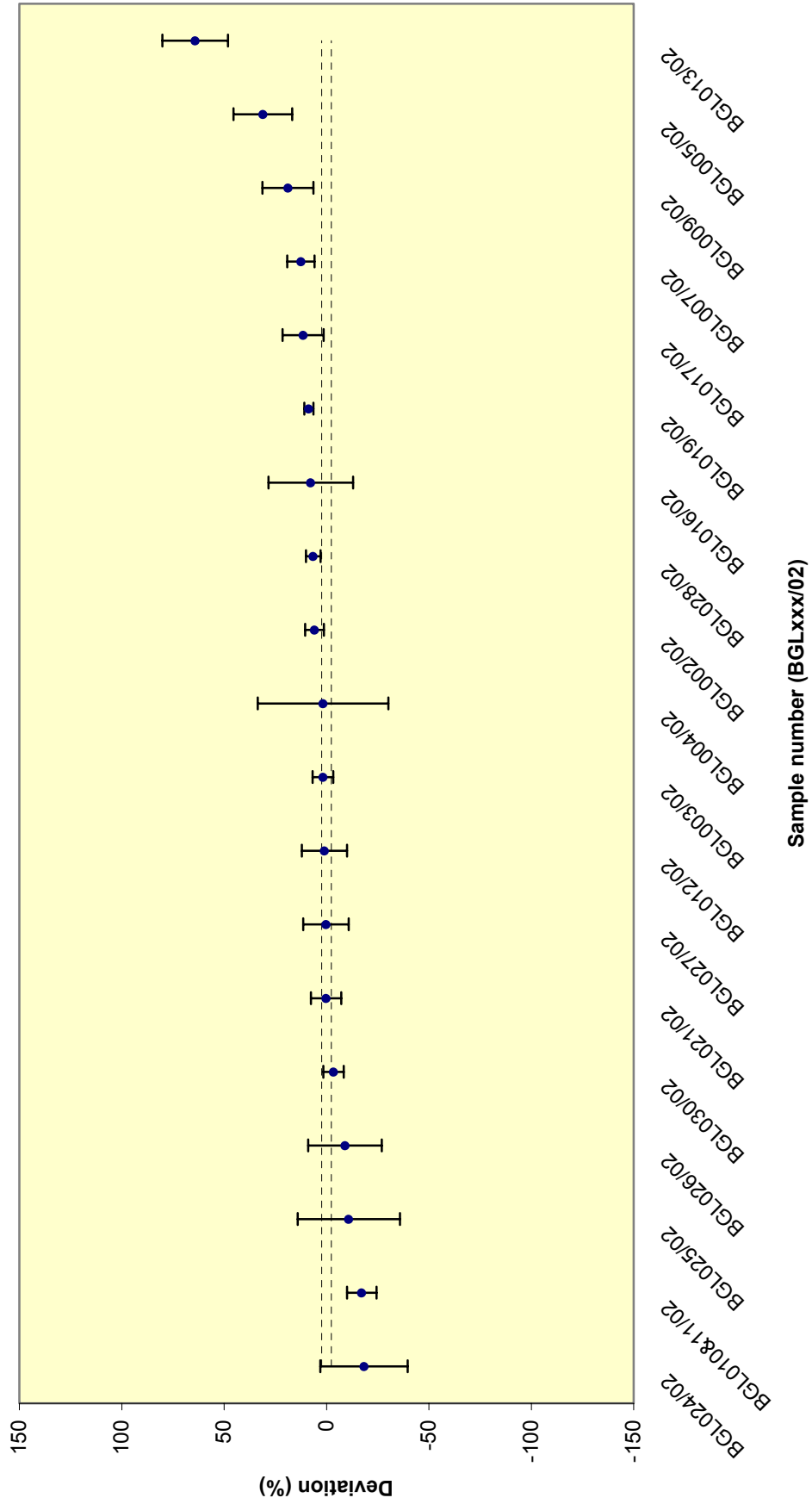
Figure 53 - Reported ^{155}\text{Eu} results (low level)
