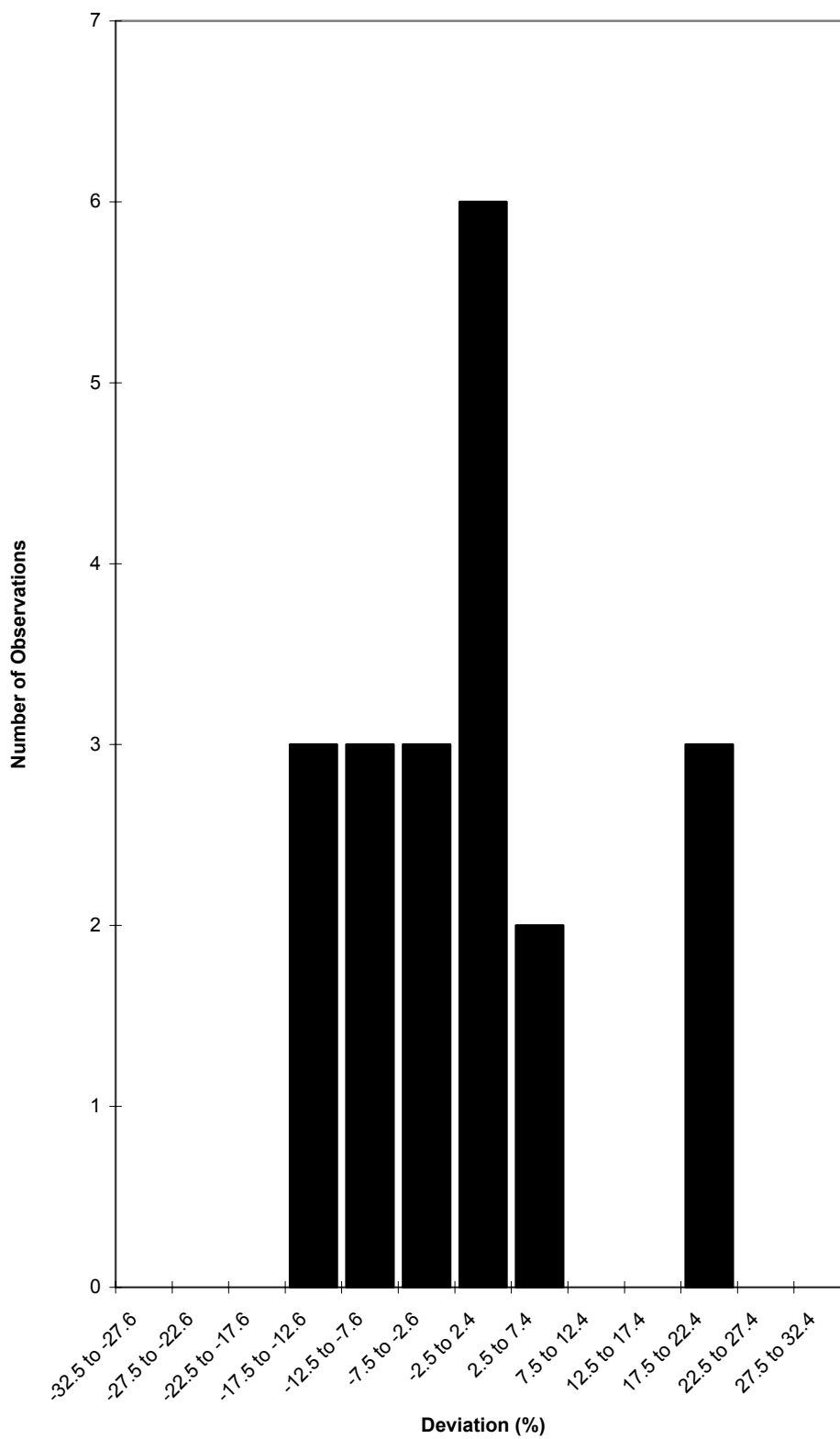
Figure 40 ^{57}\text{Co} low level results (One outside limits of plot)
