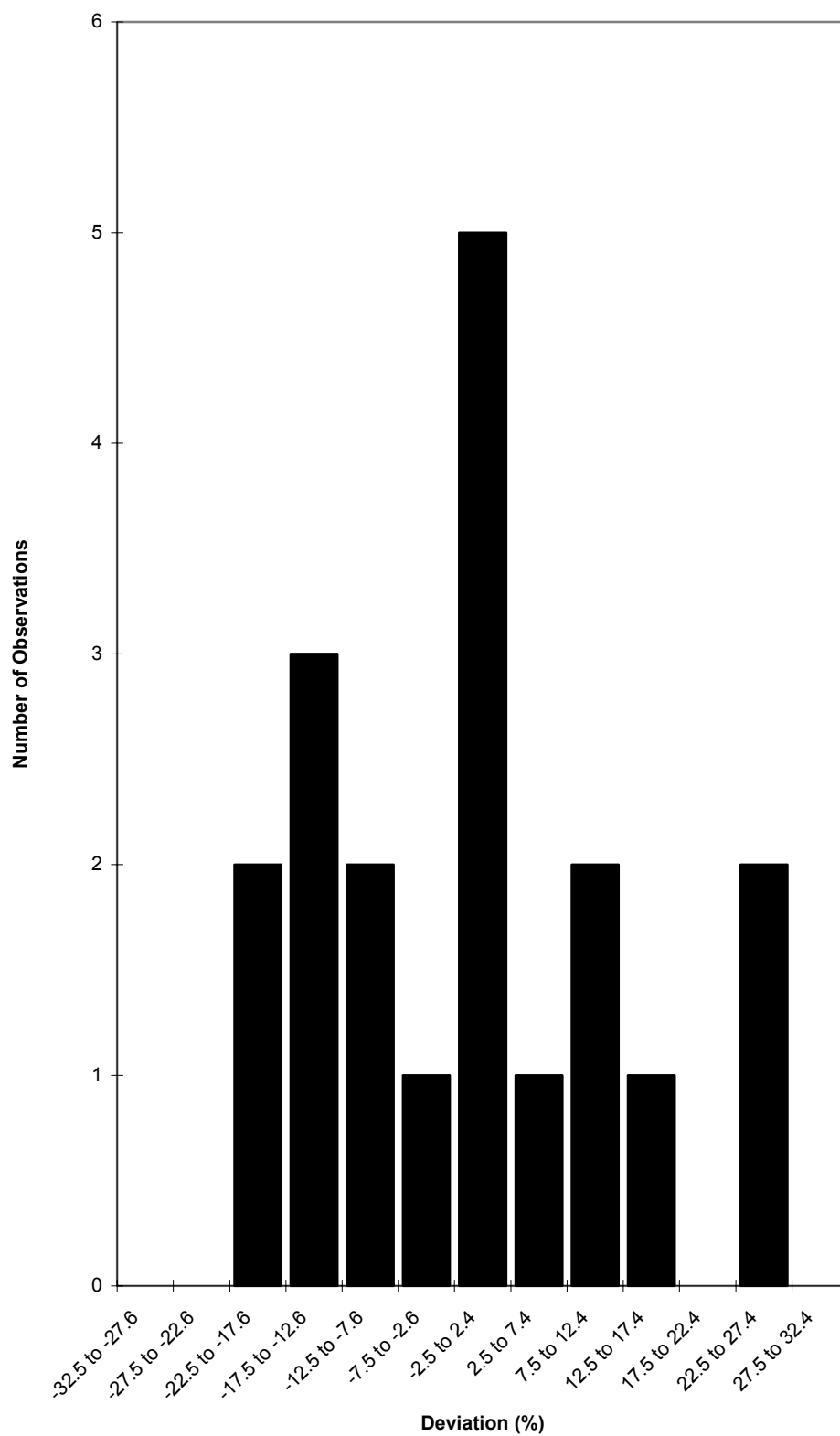
Figure 38 ^{22}\text{Na} low level results (One outside limits of plot)
