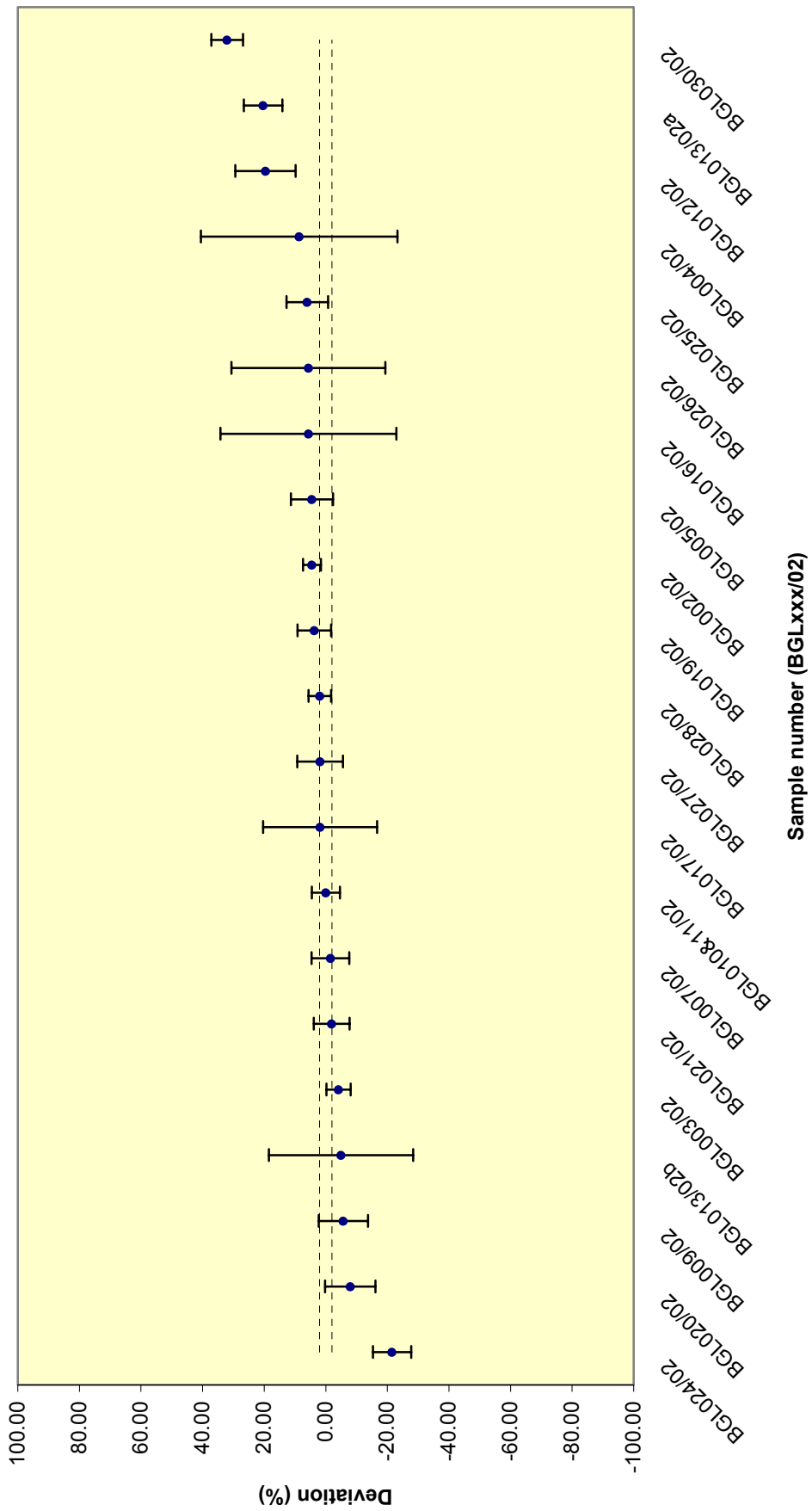
Figure 41 - Reported ^{60}\text{Co} results (low level)
