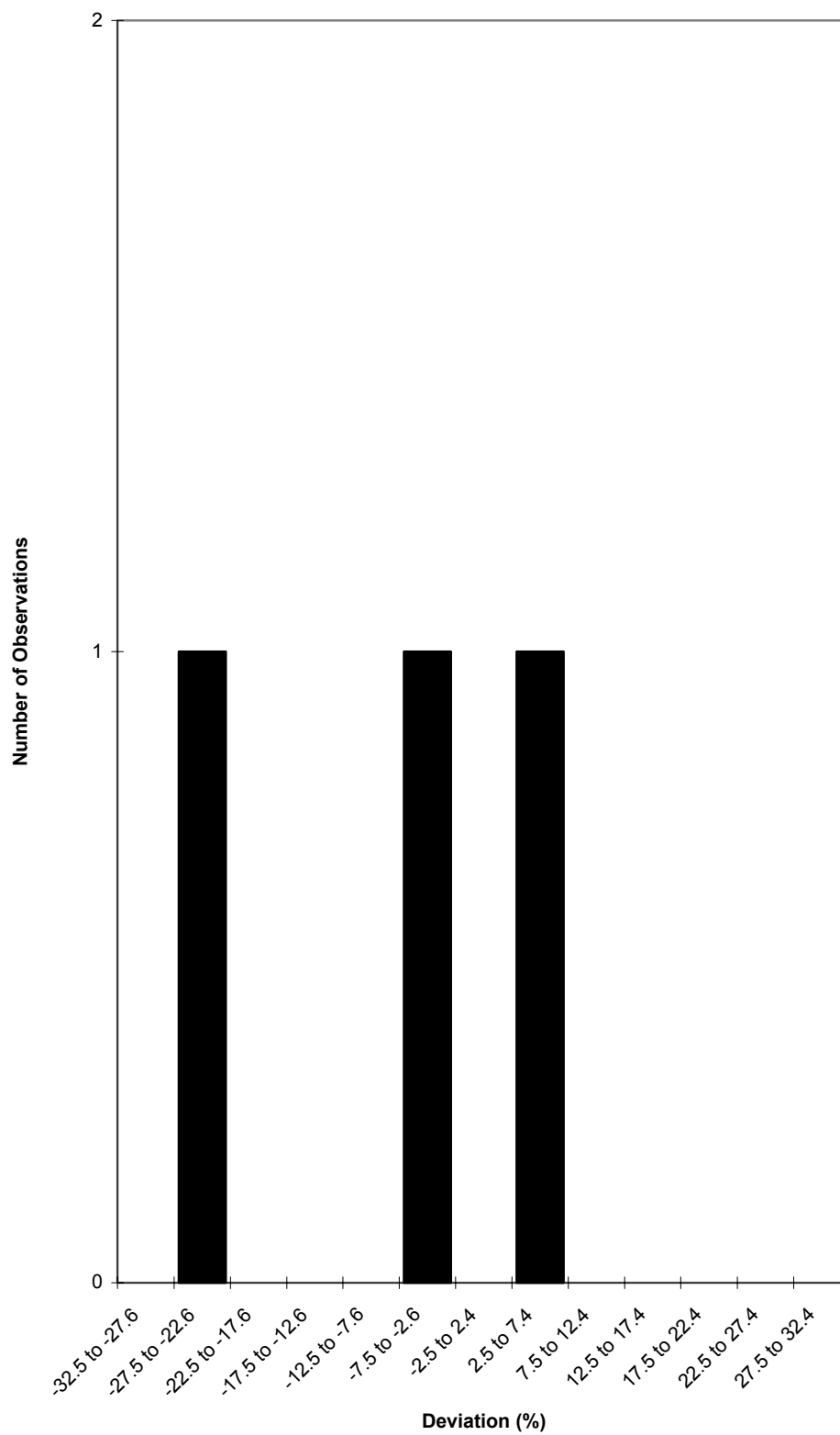
Figure 30 ^{35}\text{S} Low level results (One outside limits of plot)
