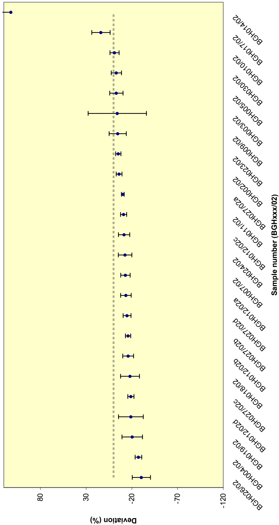
Figure 63 - Reported ^{106}\text{Ru} results (high level)
