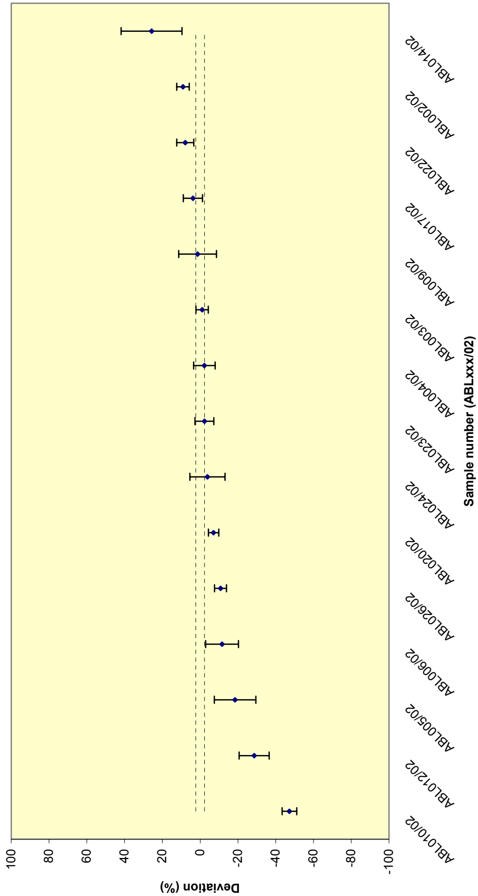
Figure 11 - Reported ^{241}\text{Am} results (low level)
