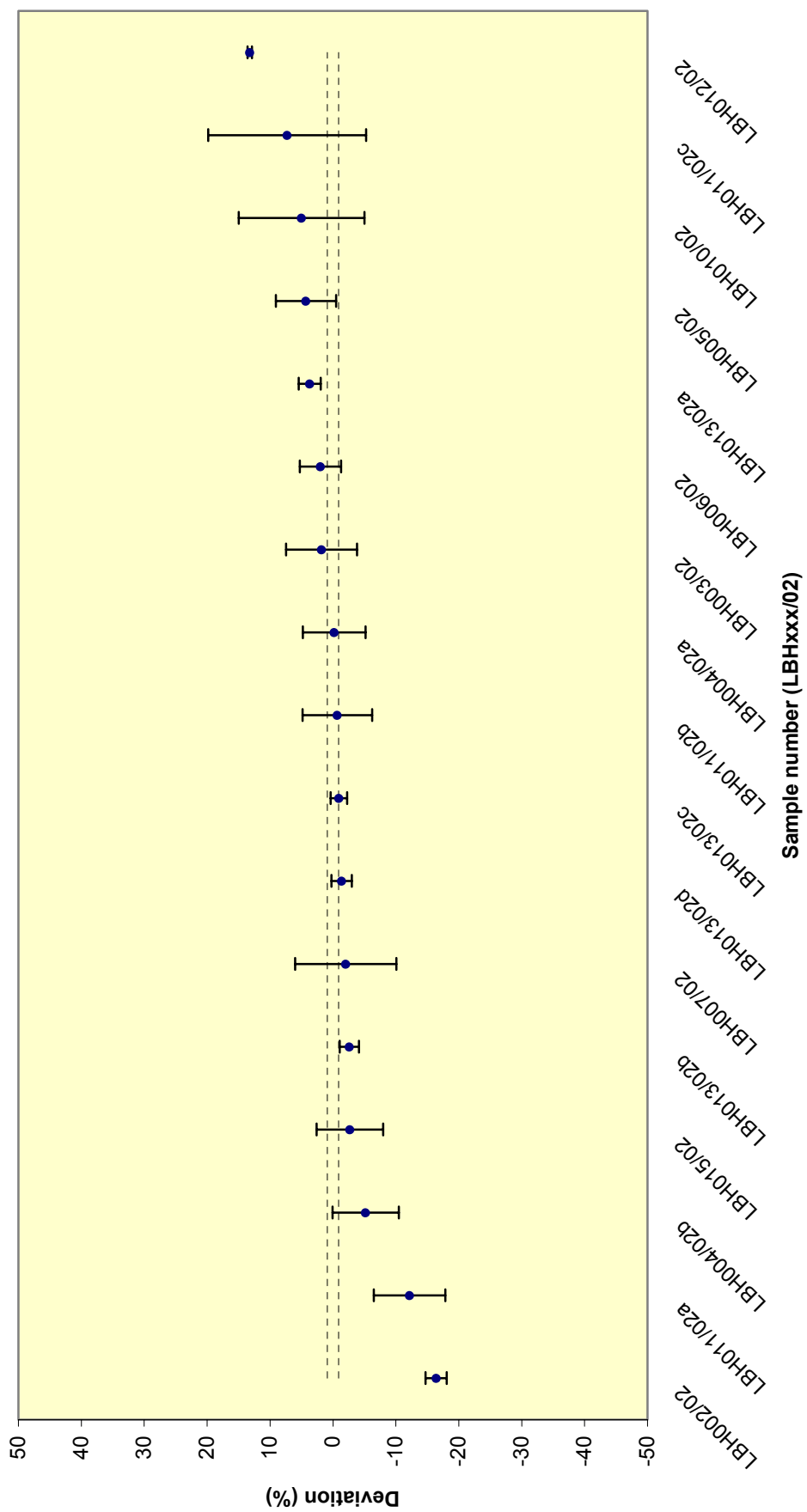
Figure 31 - Reported ^3\text{H} results (High level)
