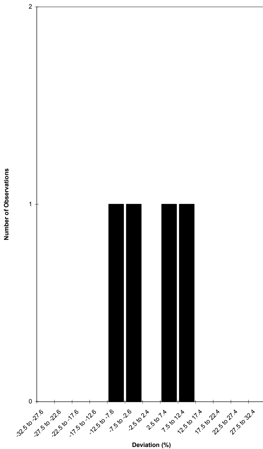
Figure 28 ^{14}\text{C} Low level results (One outside limits of plot)
