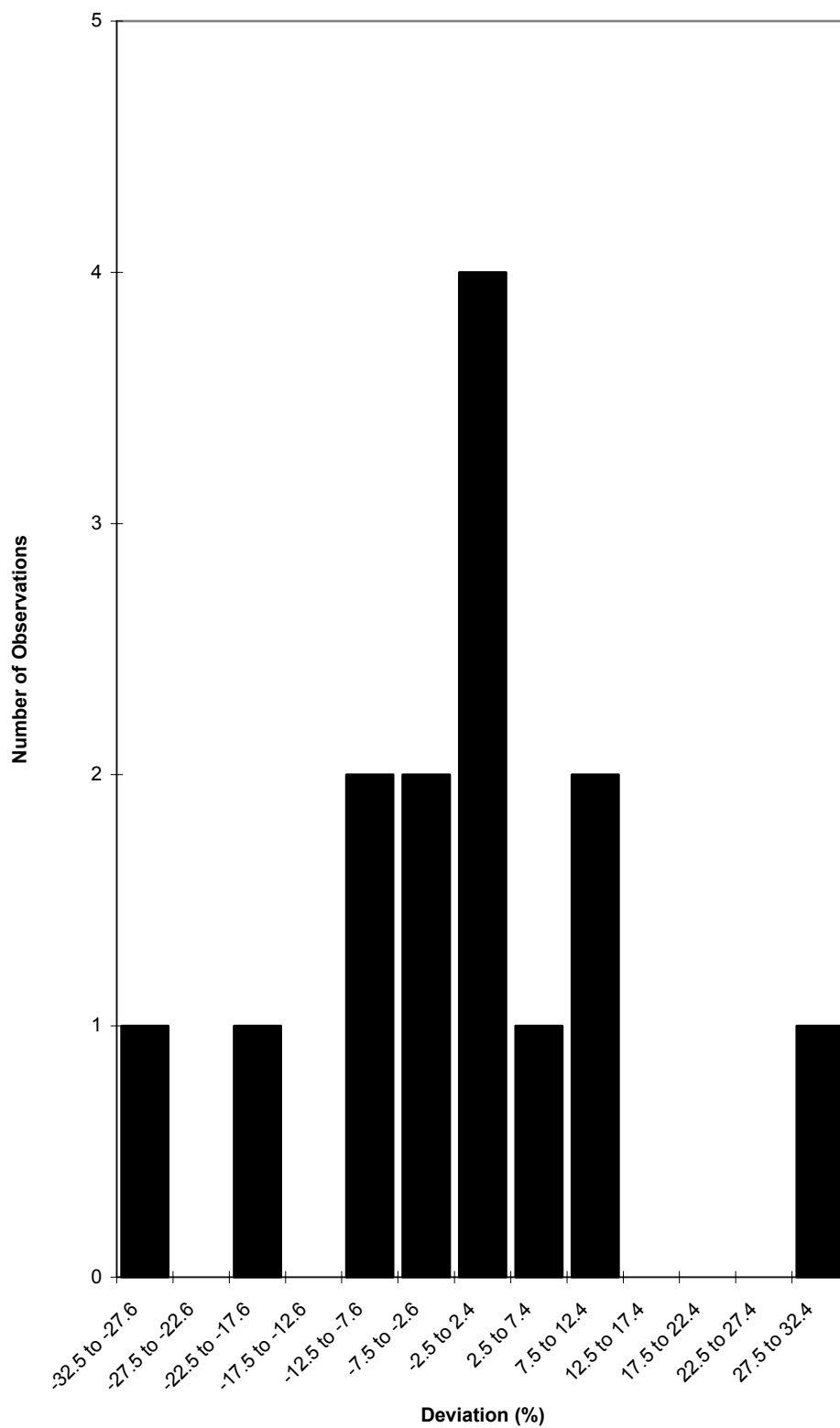
Figure 12 241 Am low level results (One outside limits of plot)
