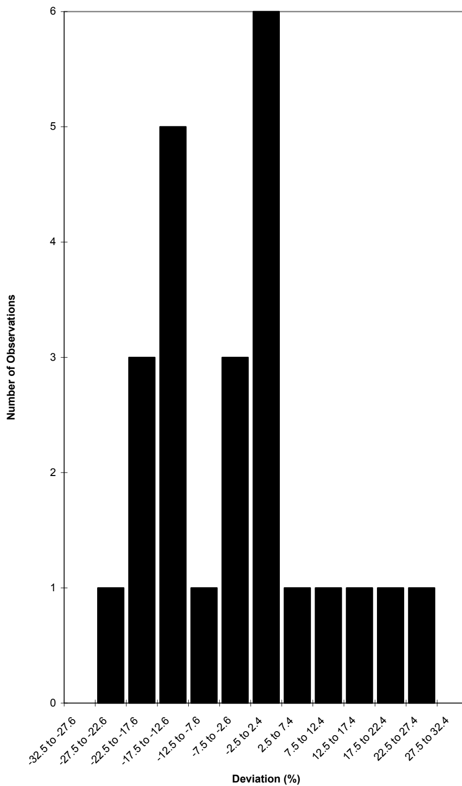
Figure 56 ^{22}\text{Na} high level results (One outside limits of plot)
