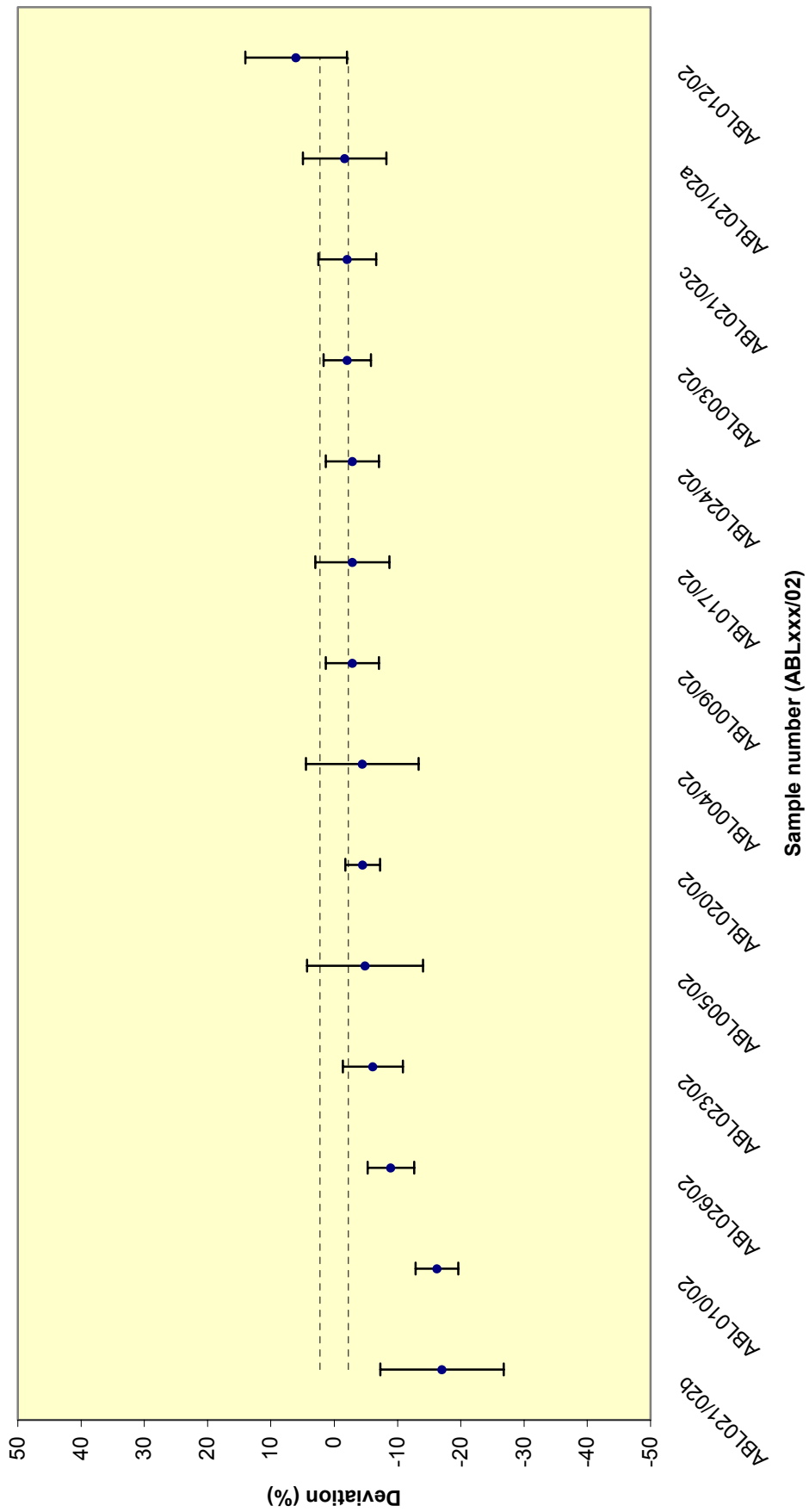
Figure 7 - Reported ^{238}\text{Pu} results (low level)
