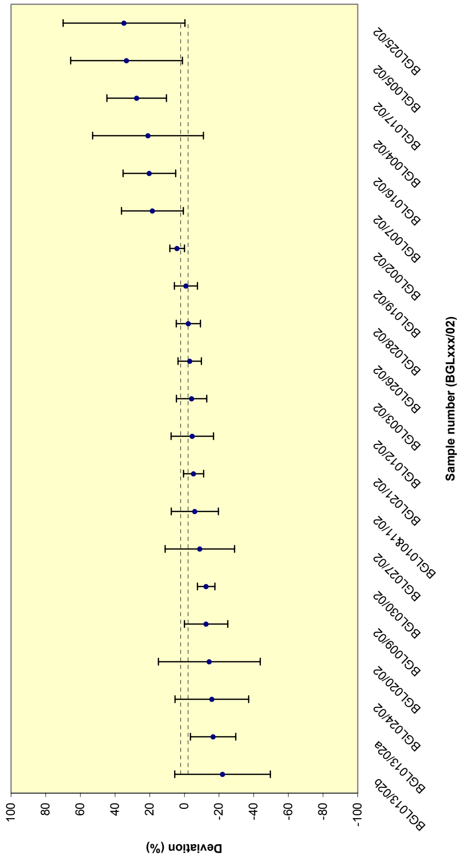
Figure 51 - Reported ^{154}\text{Eu} results (low level)
