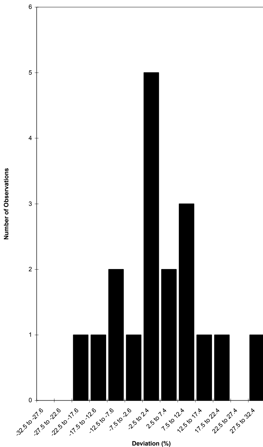
Figure 54 ^{155}\text{Eu} low level results (One outside limits of plot)
