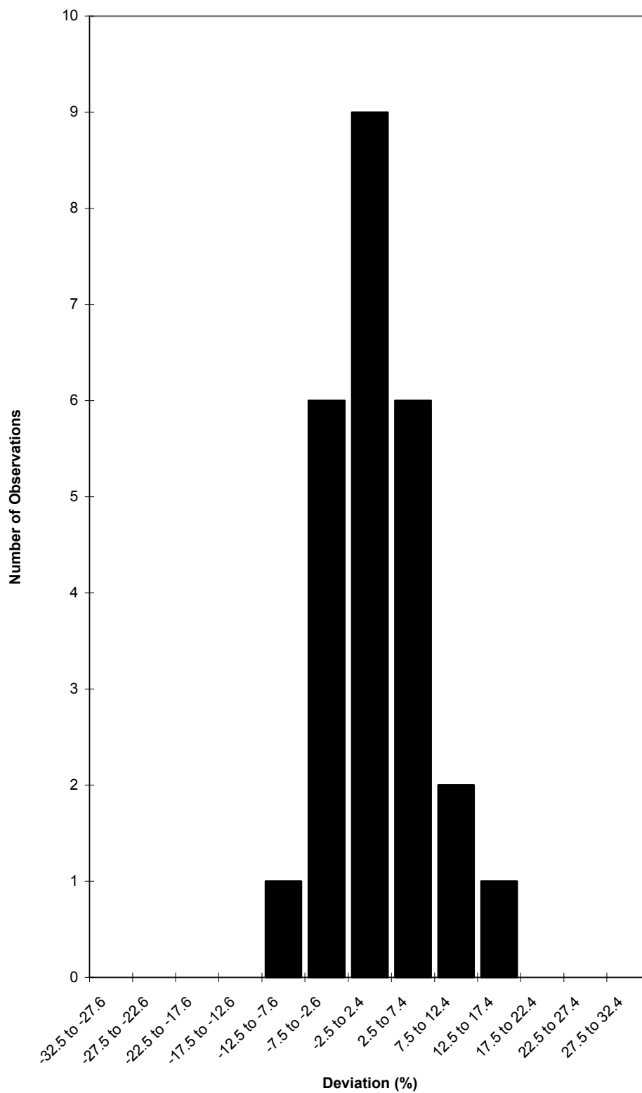
Figure 68 ^{137}\text{Cs} high level results (One outside limits of plot)
