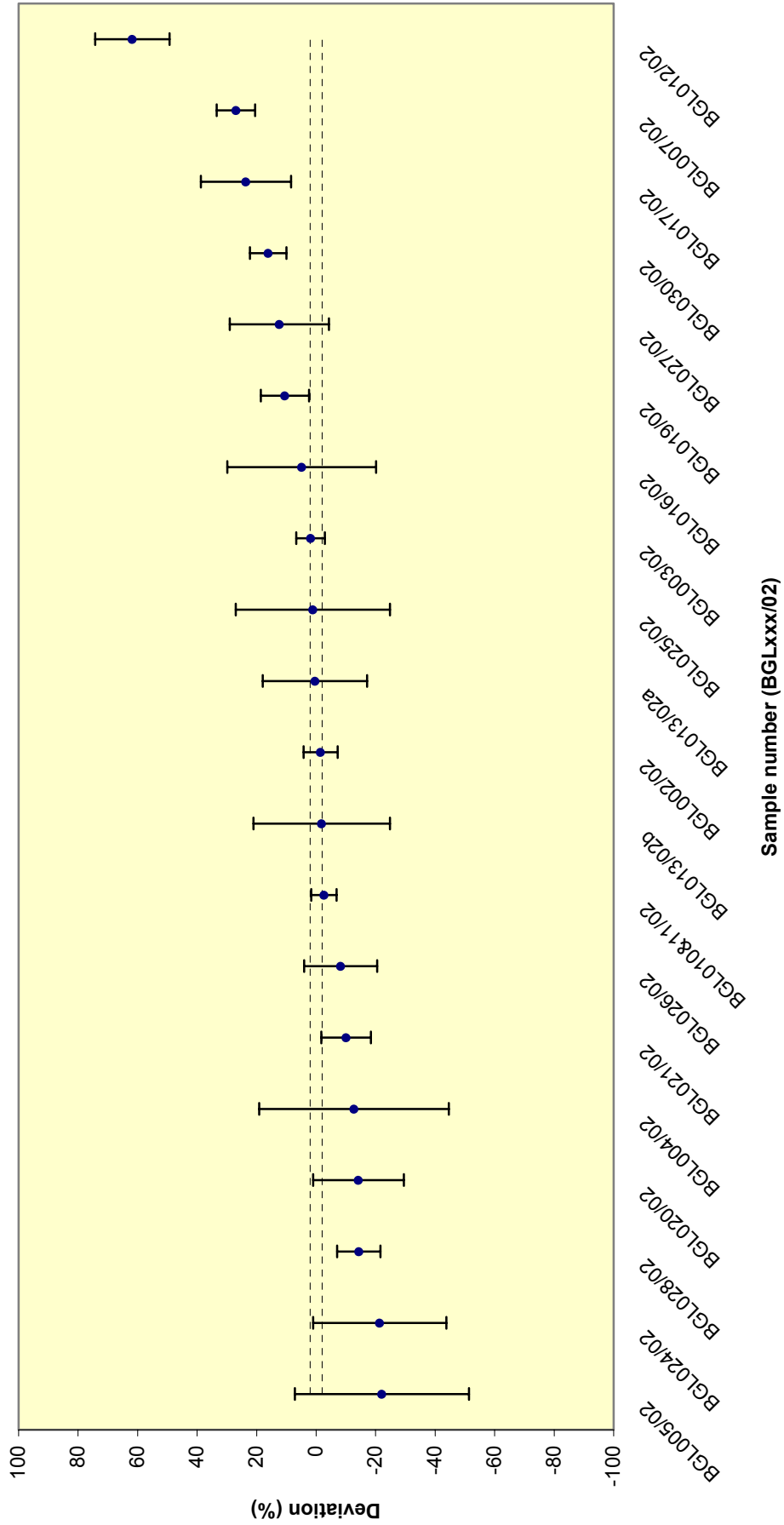
Figure 37 - Reported ^{22}\text{Na} results (low level)
