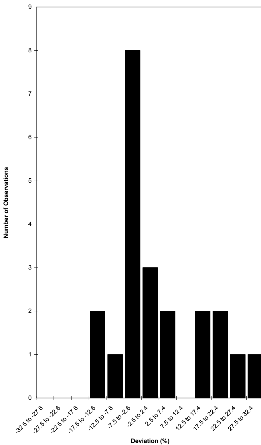
Figure 62 ^{95}\text{Zr} high level results (Three outside limits of plot)
