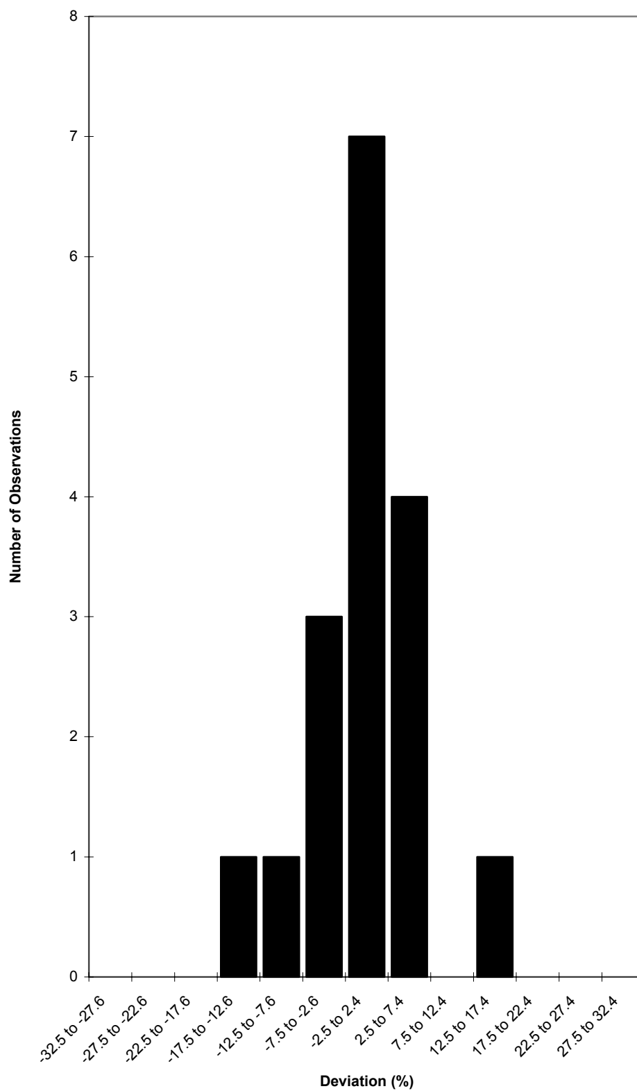
Figure 32 ^3\text{H} High level results (One outside limits of plot)
