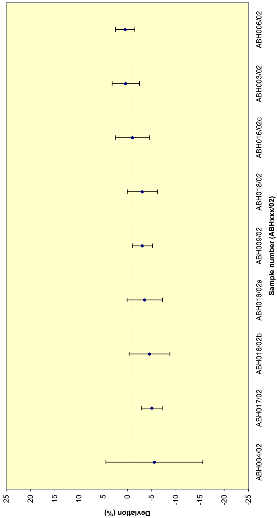
Figure 21 - Reported ^{239}\text{Pu} results (high level)
