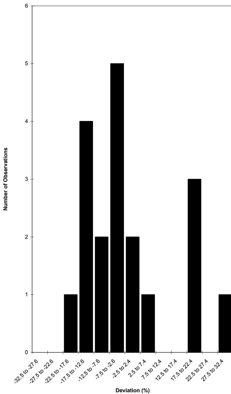
Figure 52 ^{154}\text{Eu} low level results (Two outside limits of plot)
