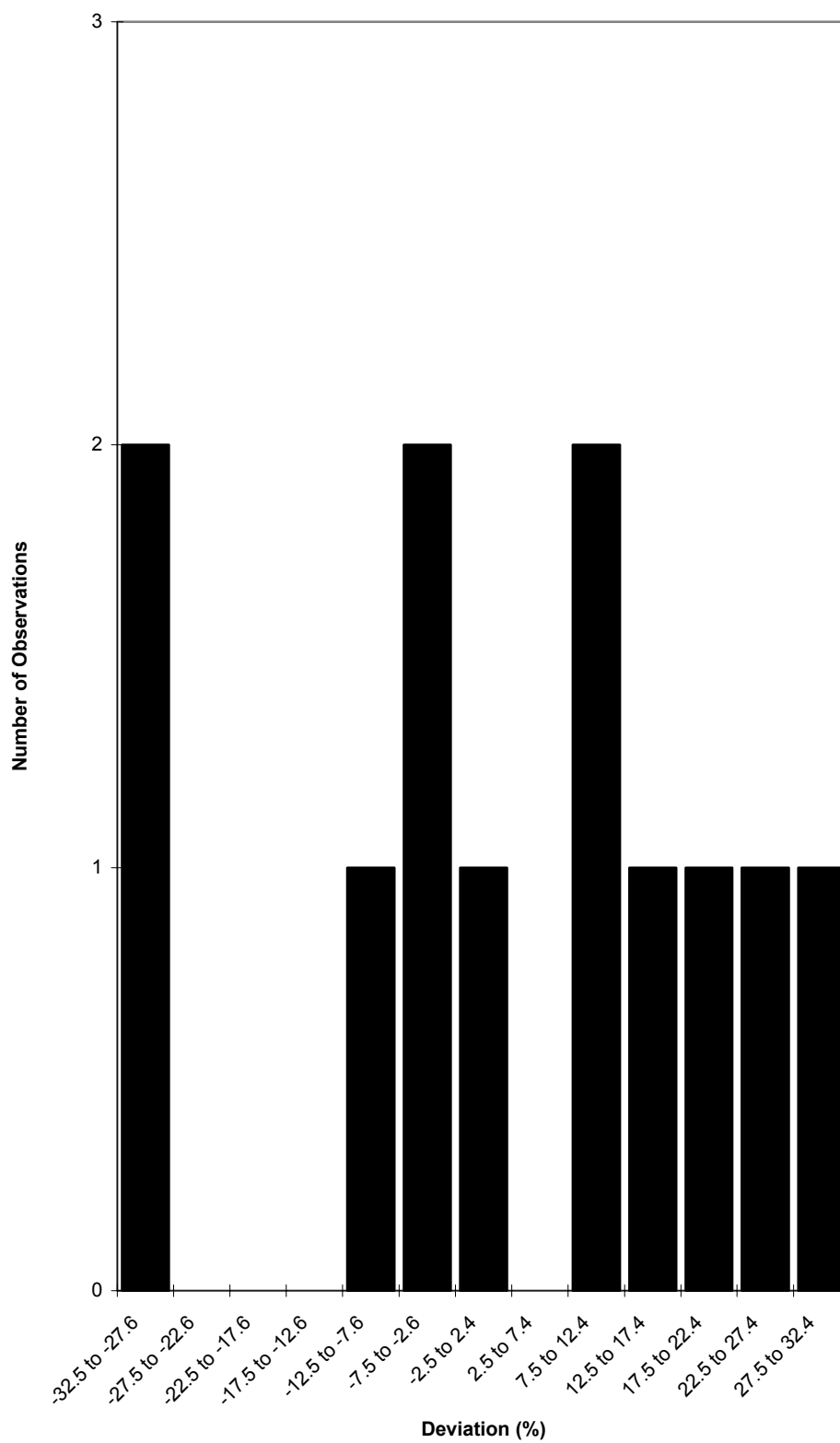
Figure 44 ^{95}\text{Zr} low level results (Five outside limits of plot)
