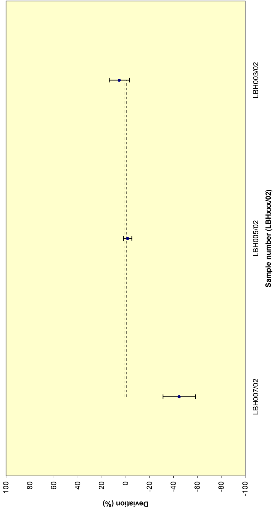
Figure 35 - Reported 35 S results (High level)
