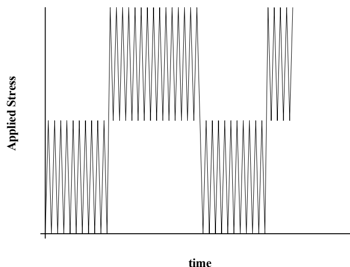
Figure 6: Blocking of constant amplitude cyclic stresses.
