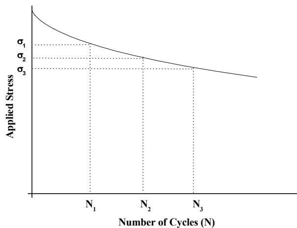
Figure 5: Schematic of Palmgren-Miner rule.
