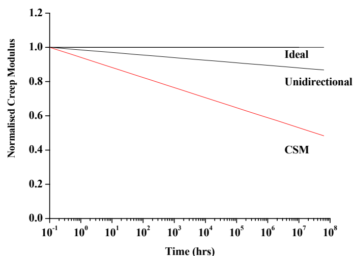
Figure 9: Normalised creep modulus for composite materials loaded in tension
