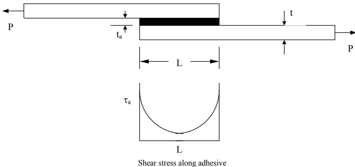
Figure A2.1: Schematic of single-lap joint.
