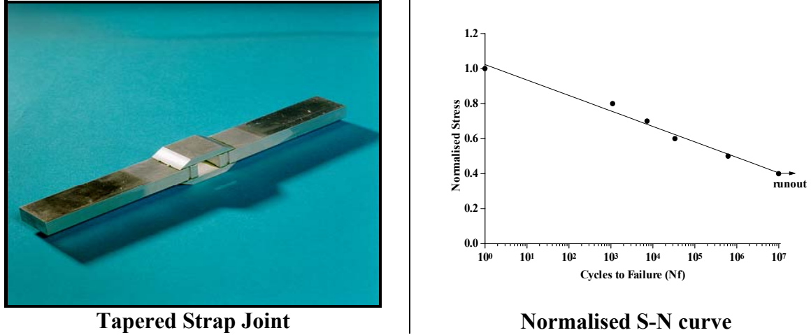
Figure 3: S-N data for 5251 aluminium alloy/AF126-2 epoxy tapered strap joints [2].
