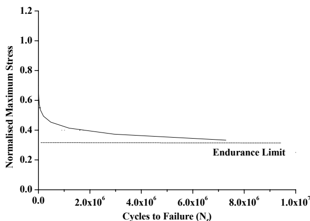
Figure 1: Typical S-N curve with fatigue or endurance limit.
