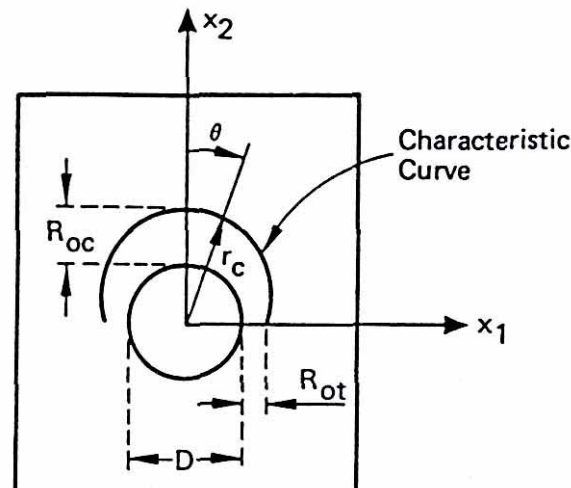
Figure 13: Whitney/Nuismer failure hypothesis [37].
