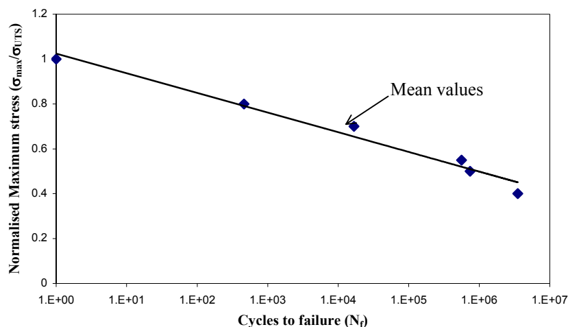
Figure 14: S-N curve for pin bearing woven glass-fibre/epoxy [42].
