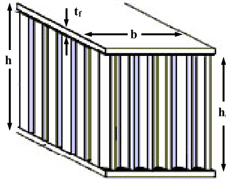
Figure 16: Sandwich panel with dimensions.
