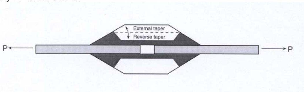
Figure 11: Bevelled strap joint.
