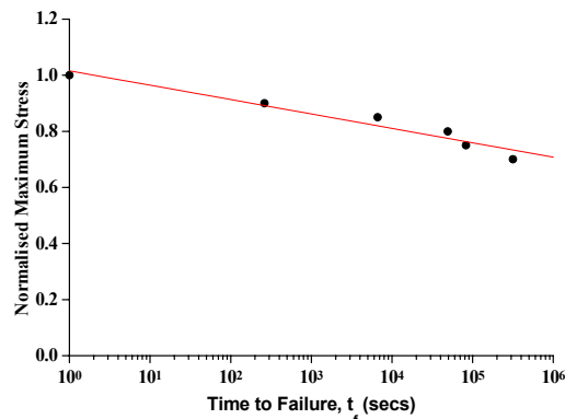
Figure 10: Creep rupture of 5251 aluminium alloy/AF126-2 epoxy tapered strap joints.
