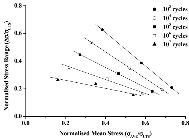
Figure 4: Stress amplitude-life plots for different mean stress values for E-glass/913 [3].
