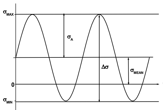
Figure 2: Stress parameters for constant amplitude sinusoidal stress-time cyclic loading.
