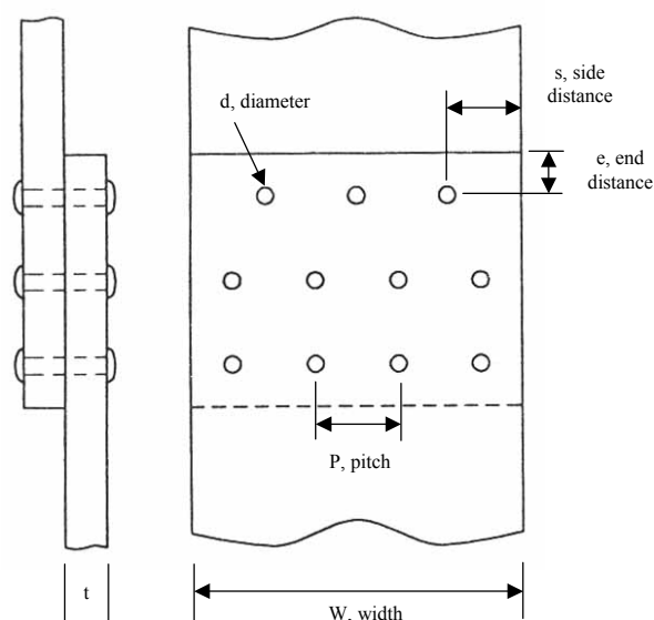
Figure 12: Multi-array bolted joint with commonly used terminology.
