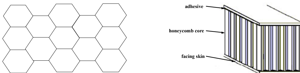
Figure 15: Sandwich structure with honeycomb core.
