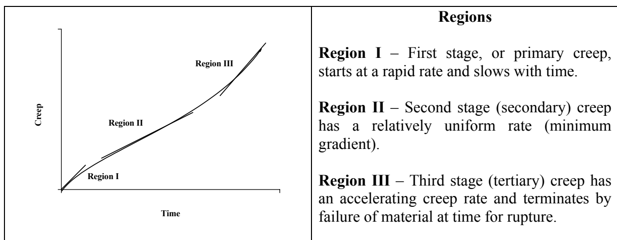
Figure 8: Creep versus time plot.
