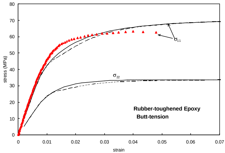
Fig 9 Comparison of the measured ( \blacklozenge ) and predicted curves of \sigma_{11} versus \epsilon_{11} for a butt-joint tension test using the Gaussian (---) and stretched-exponential (—) void nucleation functions respectively. Also shown are the predicted variations of lateral stress \sigma_{22} against \epsilon_{11} .
