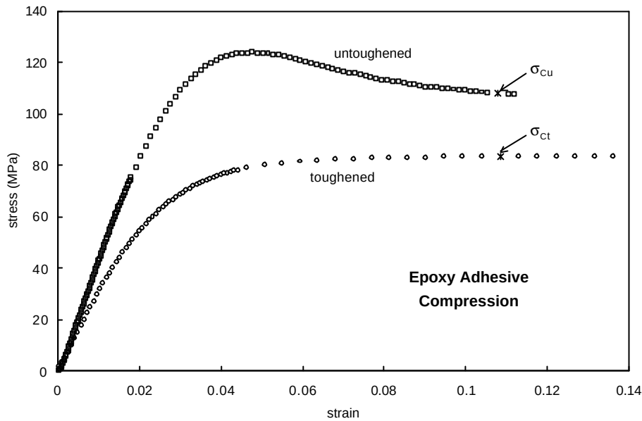
Fig 1 True stress versus true strain curves obtained under uniaxial compression for the rubber-toughened Epoxy adhesive and for the untoughened resin without rubber. Stresses \sigma_{Ct} and \sigma_{Cu} were used in determining the value of the parameter k .
